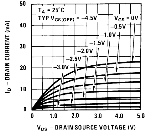
Figure 2. Common Drain-Source
