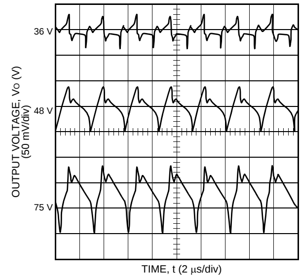
Figure 8. Typical JAHW100F Output Ripple Voltage at Room Temperature and I_o = I_{o, \max}
