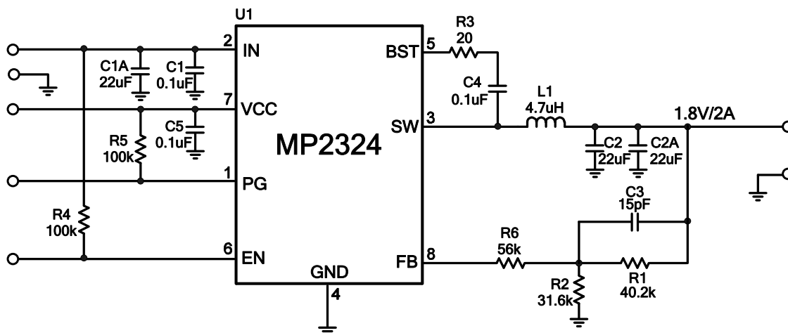
Figure 11: V_o=1.8V , I_o=2A
