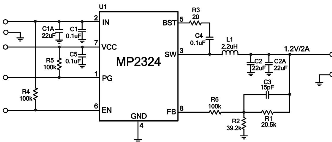
Figure 12: V_o=1.2V , I_o=2A
