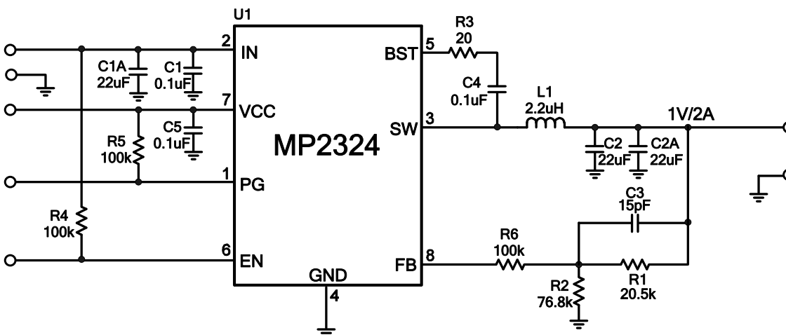
Figure 13: V_o=1V , I_o=2A
