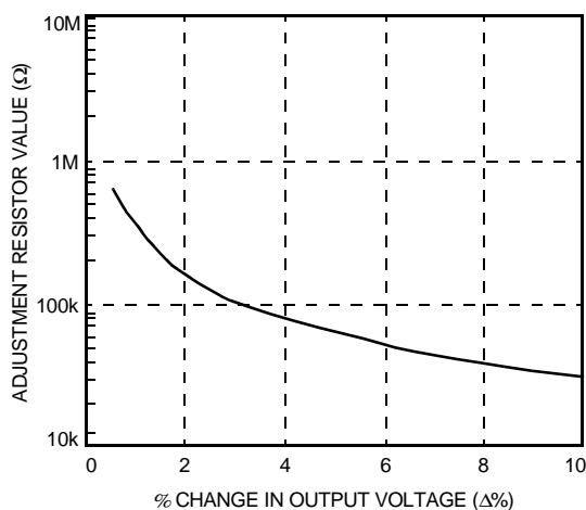
Figure 22. Resistor Selection for Increased Output Voltage
