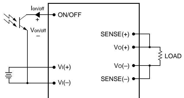
Figure 17. Remote On/Off Implementation
