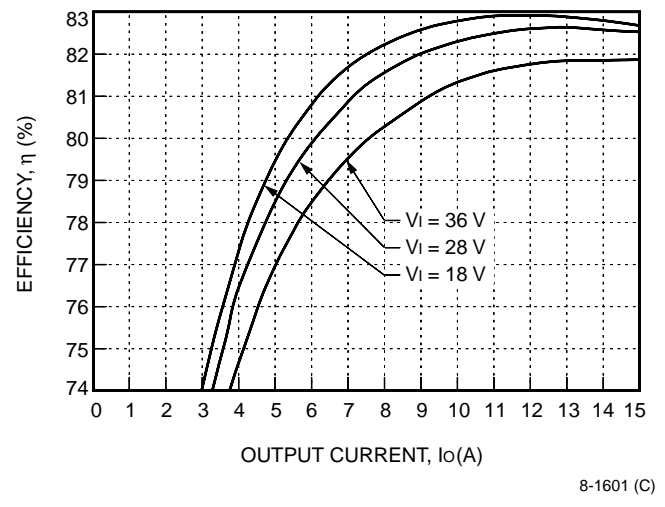
Figure 8. Typical JC075A Converter Efficiency vs. Output Current at Room Temperature
