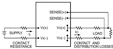
Figure 18. Effective Circuit Configuration for Single-Module Remote-Sense Operation
