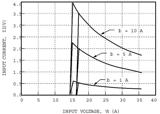
Figure 1. Typical JC050A Input Characteristics at Room Temperature
