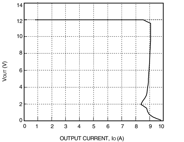
Figure 6. Typical JC100B Output Characteristics at Room Temperature, V_{IN} = 28\text{ V}
