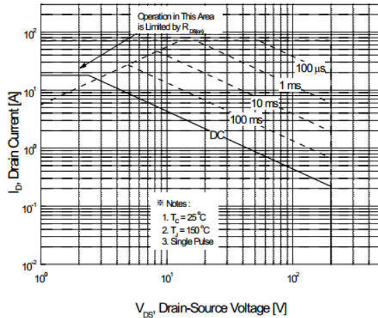
Maximum Safe Operating Area For JCS640F
