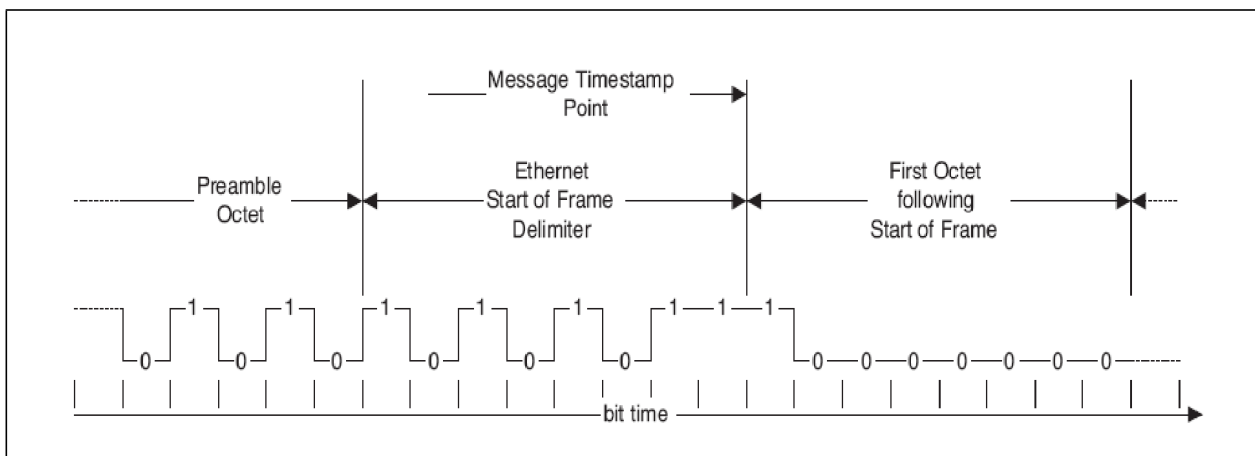
Figure 7-39 Time Stamp Point
