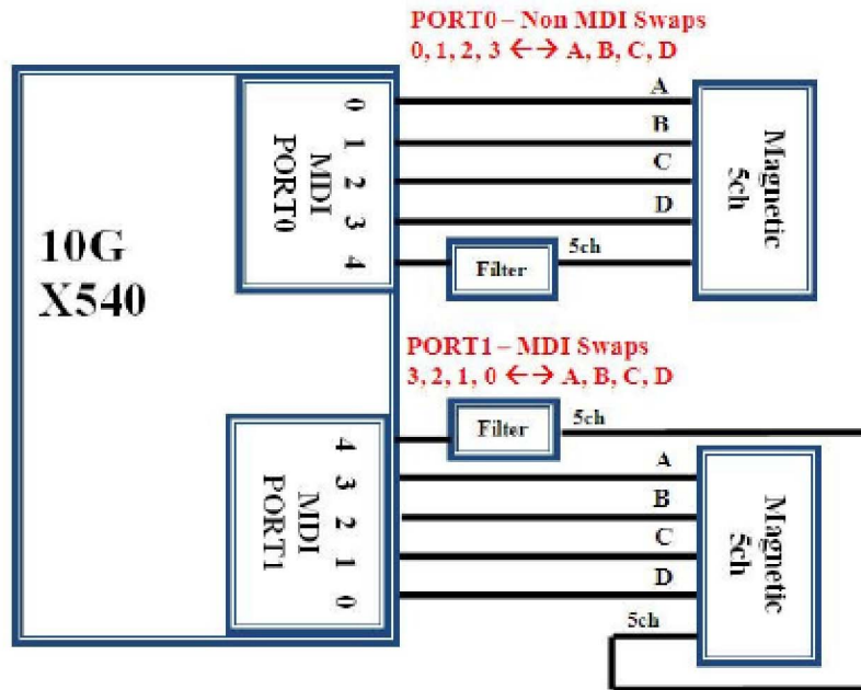
Figure 13-7. PHY AFE_LINE Lane Swap Configuration
