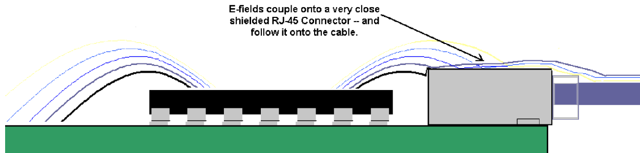
Figure 13-3. Effect of Device Placed Less Than One Inch from the RJ-45 Connector
