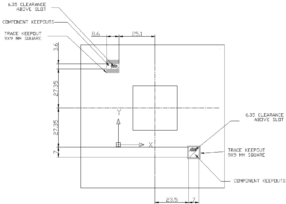
Figure 14-2 Twinville Heatsink Keep Out Restrictions (Bottom Side Keep Out)
