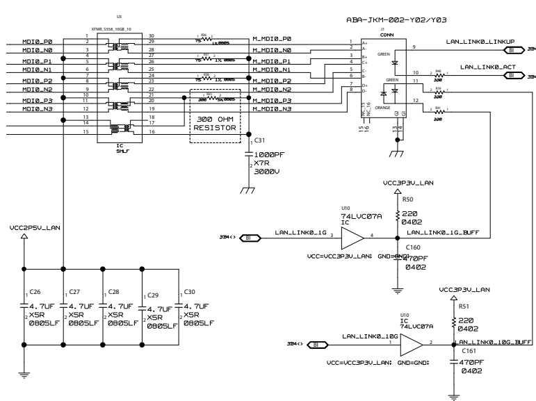
Figure 13-17. LED Connectivity
