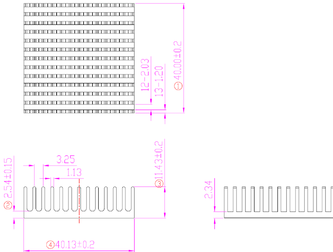
Figure 14-3 Twinville Extruded Heatsinks (11.43 mm Height Passive Heat Sink (AAVID Thermalloy Profile# 72845))
