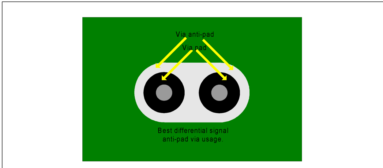
Figure 13-31. Best Differential Signals Via Anti-Pads
