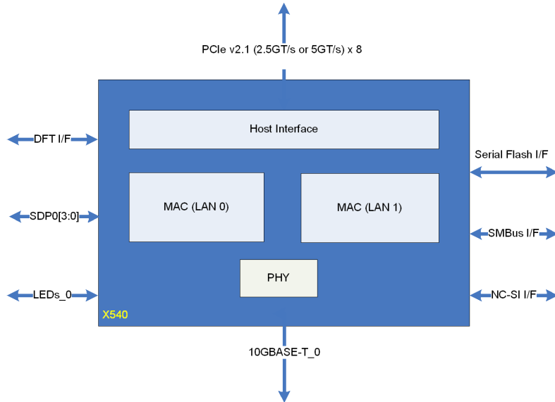
Figure 1-3 X540 External Interfaces Diagram (Single Port)
