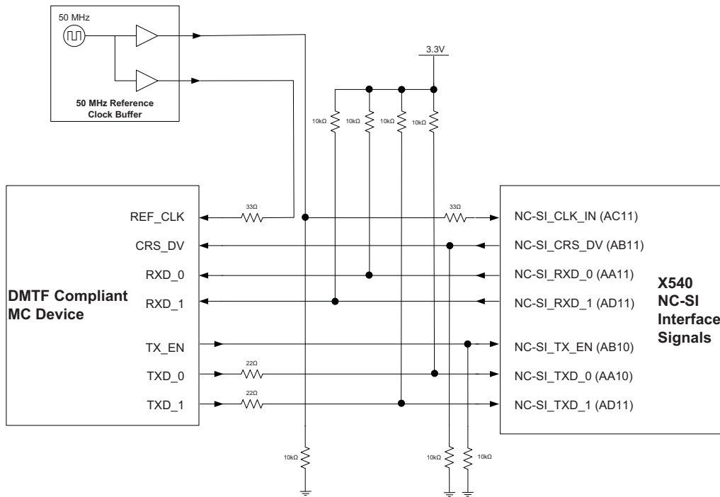
Figure 13-14. NC-SI Connections to an External MC
