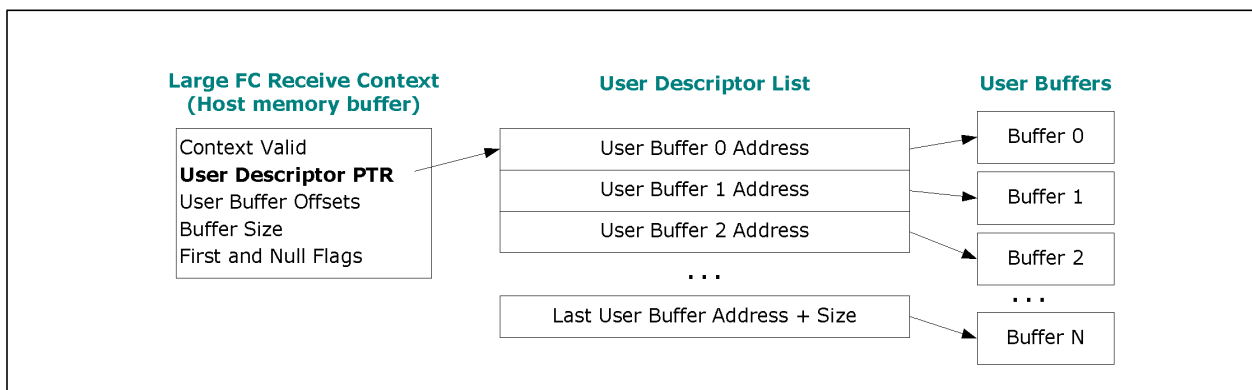
Figure 7-56 Large FC Receive Context Related to the User Buffers
