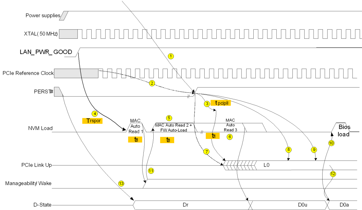
Figure 4-2 Power-Up Timing Diagram
