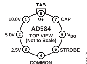
Figure 1. 8-Pin TO-99
