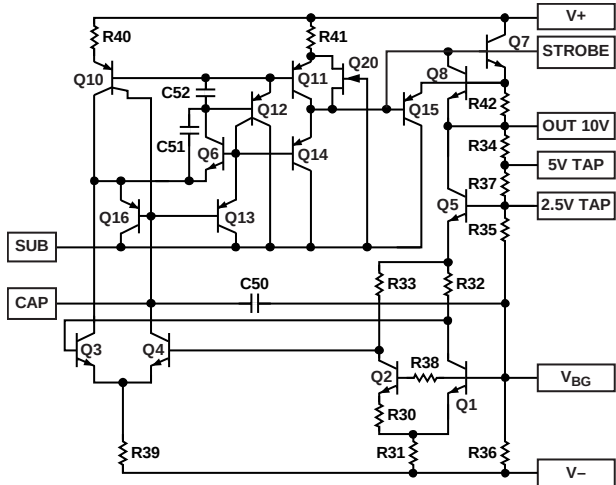
Figure 5. Schematic Diagram
