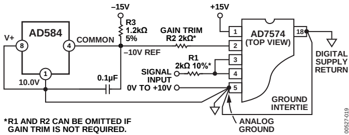
Figure 17. AD584 as -10\text{ V} Reference for CMOS ADC
