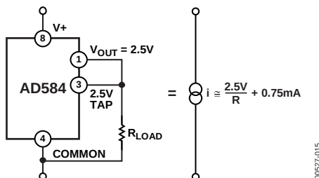
Figure 14. A Two-Component Precision Current Limiter
