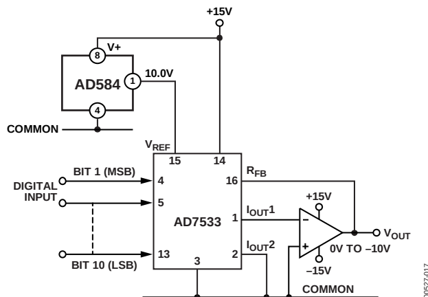
Figure 16. Low Power 10-Bit CMOS DAC Application
