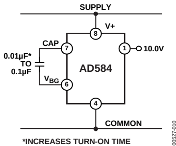
Figure 9. Additional Noise Filtering with an External Capacitor
