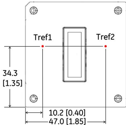
Figure 18. Case (Tref) Temperature Measurement Locations (top view).
