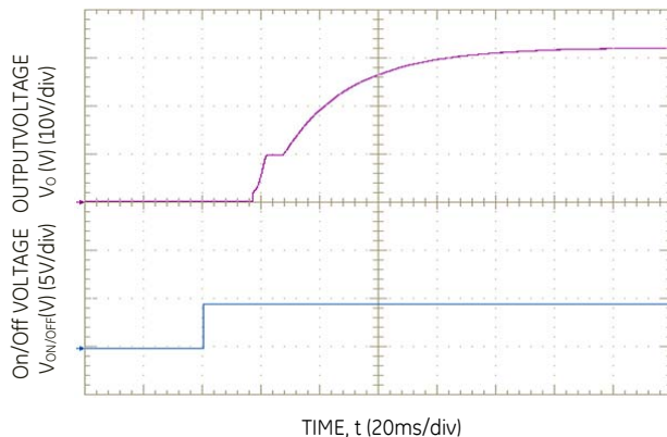
Figure 4. Typical Start-Up Using positive Remote On/Off; C_{o,ext} = 440\mu\text{F} .
