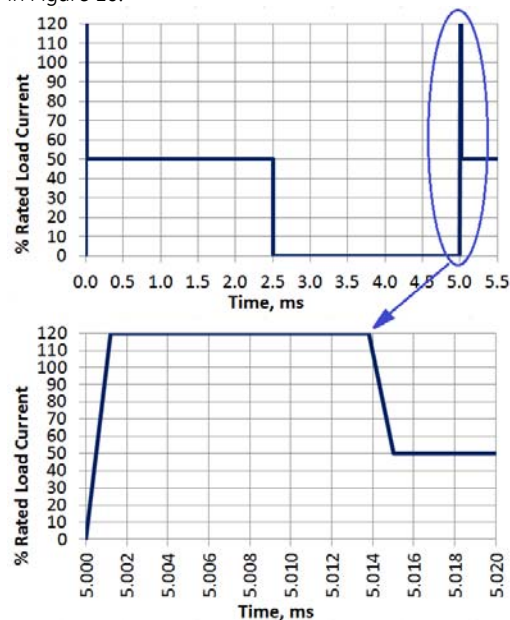
Figure 16. AC-DC Load Profile
