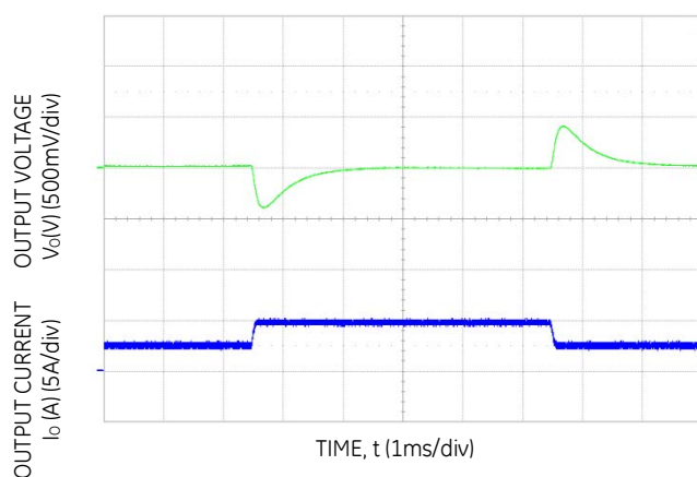
Figure 3. Dynamic Load Change Transient Response from 25% to 50% to 25% of Full Load at Room Temperature and 48 Vin; 0.1A/μS, C_{o,ext} = 440\mu\text{F} .
