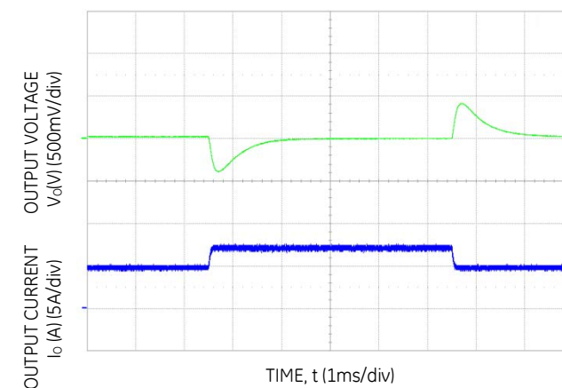
Figure 6. Dynamic Load Change Transient Response from 50 % to 75% to 50% of Full Load at Room Temperature and 48 Vin; 0.1A/μS, C_{o,ext} = 440\mu\text{F} .
