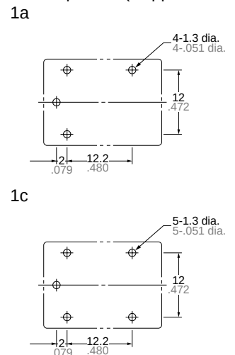
PC board pattern (Copper-side view)
