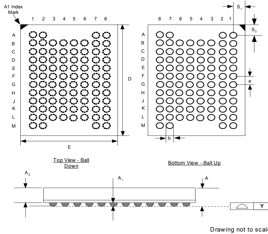
Figure 4: 64/128-Mbit, 88-ball (80 active) QUAD+ SCSP Specifications (8x10x1.2 mm)
