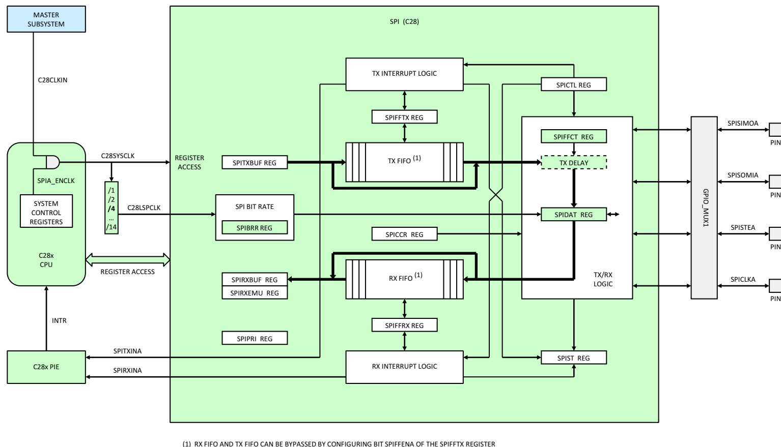
Figure 5-51. SPI (C28x)
