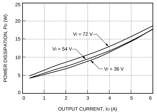
Figure 34. JW150H Power Dissipation vs. Output Current
