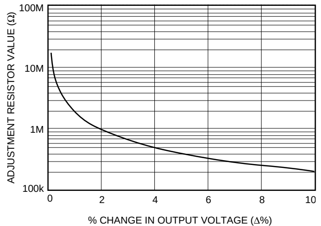
Figure 28. Resistor Selection for Increased Output Voltage
