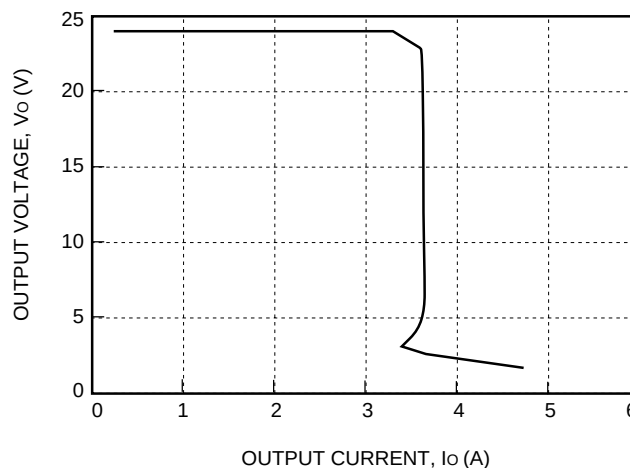
Figure 7. Typical JW075H Output Characteristics at Room Temperature
