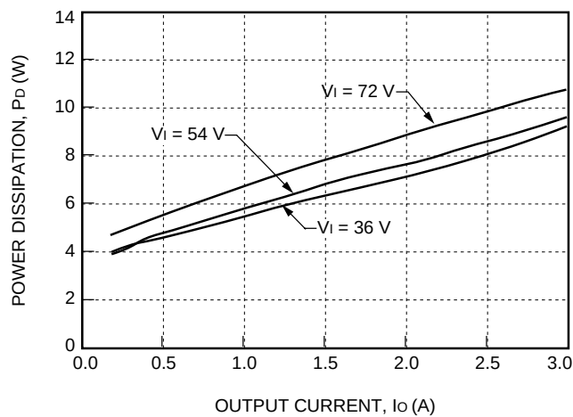
Figure 32. JW075H Power Dissipation vs. Output Current
