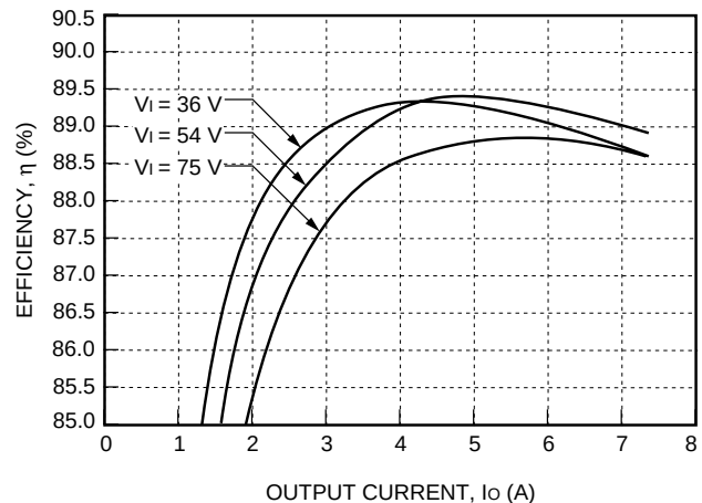
Figure 15. Typical JW175H Converter Efficiency vs. Output Current at Room Temperature
