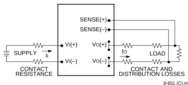
Figure 24. Effective Circuit Configuration for Single-Module Remote-Sense Operation
