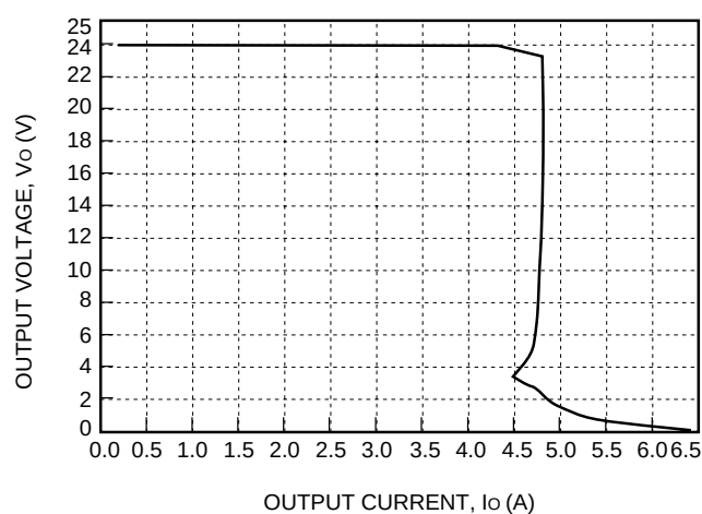
Figure 8. Typical JW100H Output Characteristics at Room Temperature
