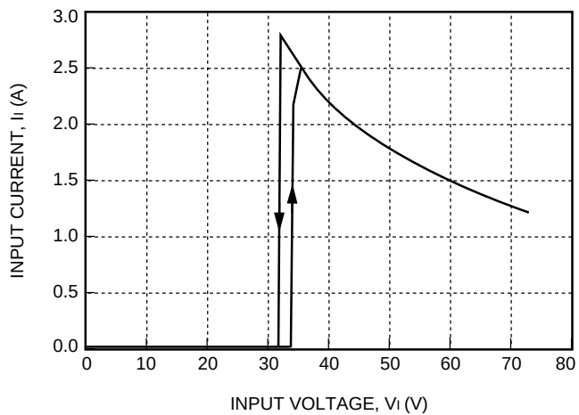
Figure 2. Typical JW075H Input Characteristics at Room Temperature
