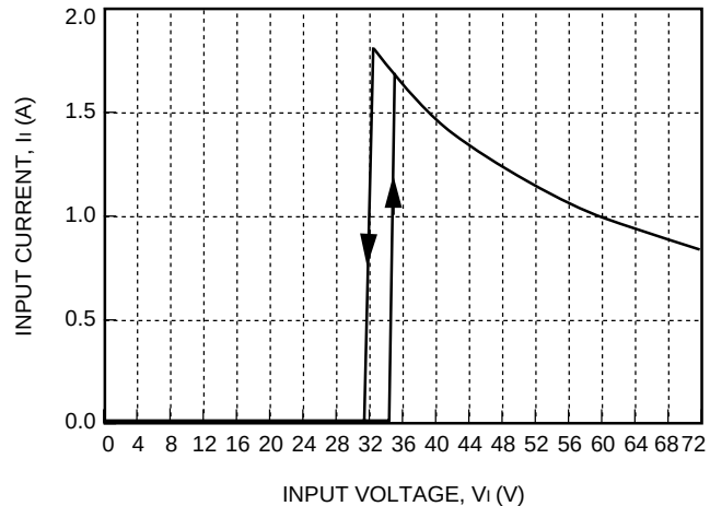
Figure 1. Typical JW050H Input Characteristics at Room Temperature
