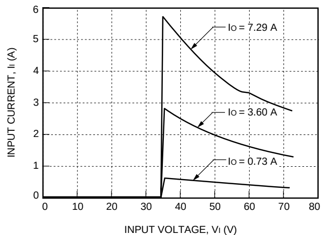
Figure 5. Typical JW175H Input Characteristics at Room Temperature
