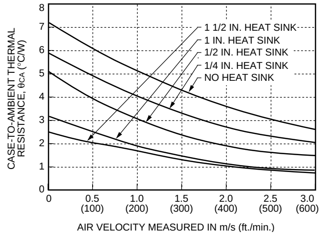
Figure 36. Case-to-Ambient Thermal Resistance Curves; Either Orientation
