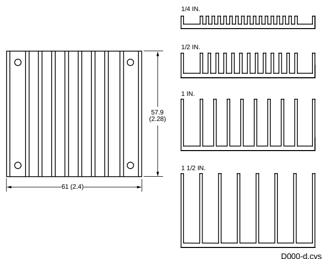
Figure 39. Transverse Heat Sink
