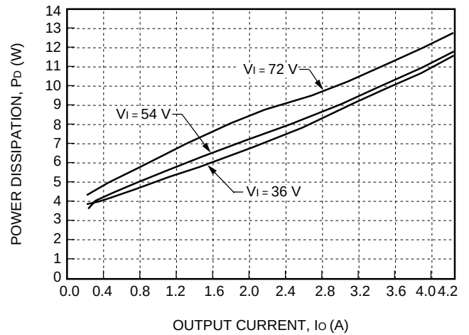
Figure 33. JW100H Power Dissipation vs. Output Current
