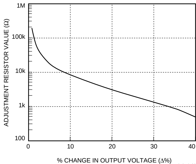
Figure 26. Resistor Selection for Decreased Output Voltage
