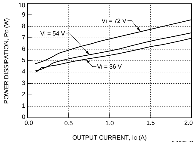
Figure 31. JW050H Power Dissipation vs. Output Current
