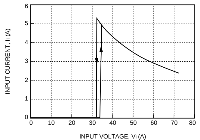
Figure 4. Typical JW150H Input Characteristics at Room Temperature
