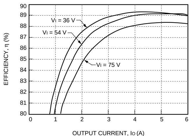
Figure 14. Typical JW150H Converter Efficiency vs. Output Current at Room Temperature
