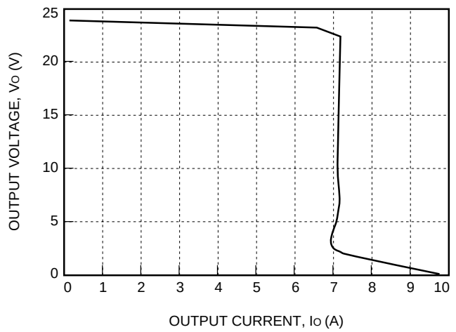
Figure 9. Typical JW150H Output Characteristics at Room Temperature
