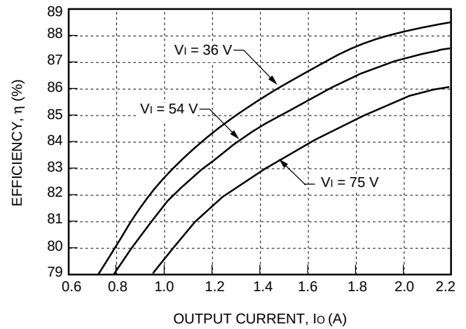
Figure 11. Typical JW050H Converter Efficiency vs. Output Current at Room Temperature
