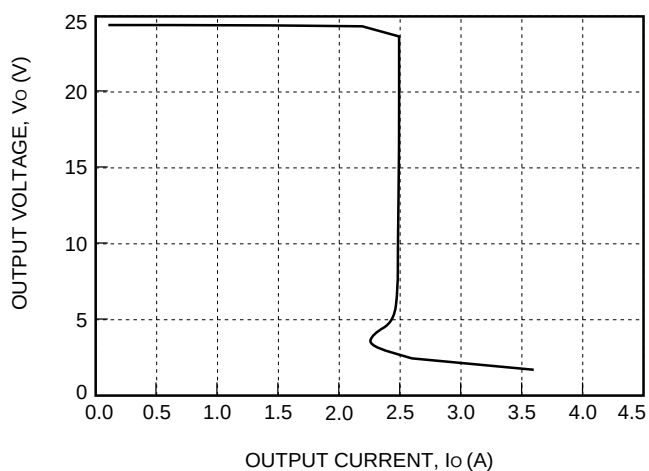
Figure 6. Typical JW050H Output Characteristics at Room Temperature
