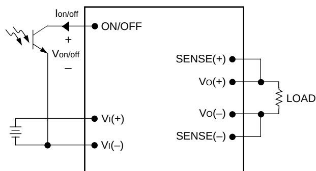
Figure 23. Remote On/Off Implementation 8-720 (C).c
