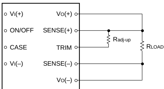
Figure 27. Circuit Configuration to Increase Output Voltage
