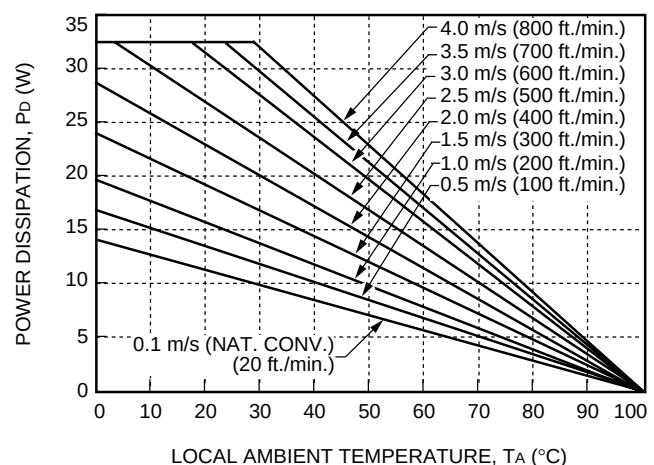
Figure 30. Forced Convection Power Derating with No Heat Sink; Either Orientation
