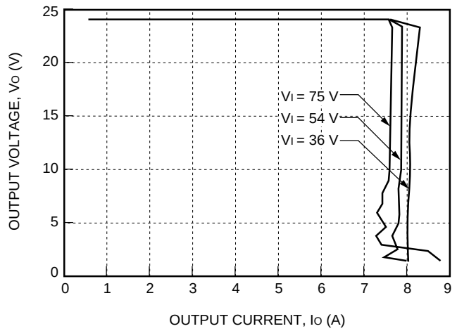
Figure 10. Typical JW175H Output Characteristics at Room Temperature
