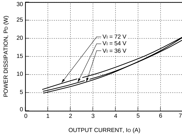
Figure 35. JW175H Power Dissipation vs. Output Current
