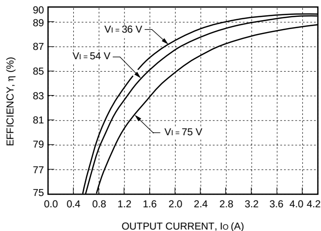
Figure 13. Typical JW100H Converter Efficiency vs. Output Current at Room Temperature
