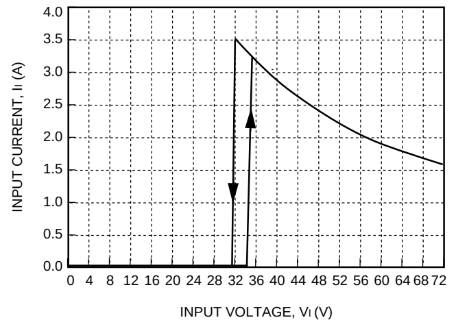
Figure 3. Typical JW100H Input Characteristics at Room Temperature
