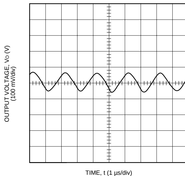
Figure 16. Typical JW150H Output Ripple Voltage at Room Temperature, 48 V Input, I_o = Full Load
