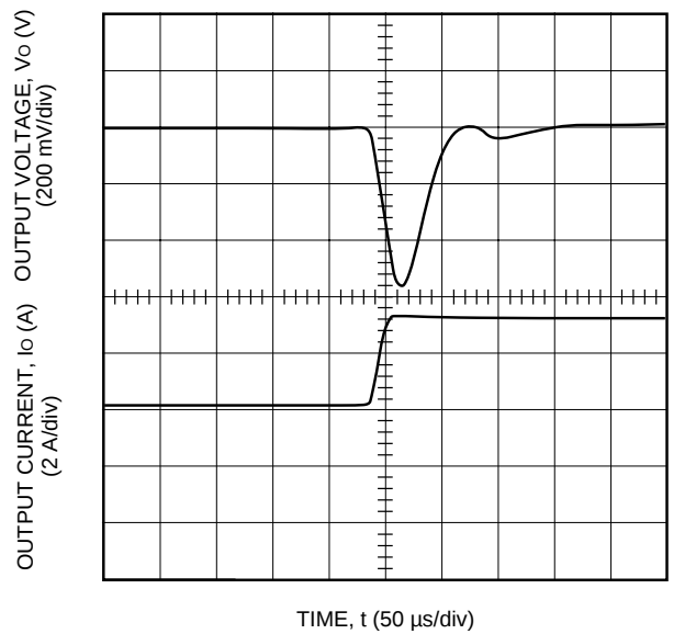
Figure 15. Typical JW150B Transient Response to Step Increase in Load from 50% to 75% of Full Load at Room Temperature and 48 V Input (Waveform Averaged to Eliminate Ripple Component.)
