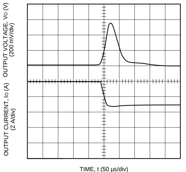
Figure 14. Typical JW150B Transient Response to Step Decrease in Load from 50% to 25% of Full Load at Room Temperature and 48 V Input (Waveform Averaged to Eliminate Ripple Component.)
