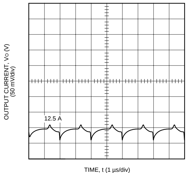
Figure 13. Typical JW150B Output Ripple Voltage at Room Temperature, 48 V Input, I_o = Full Load
