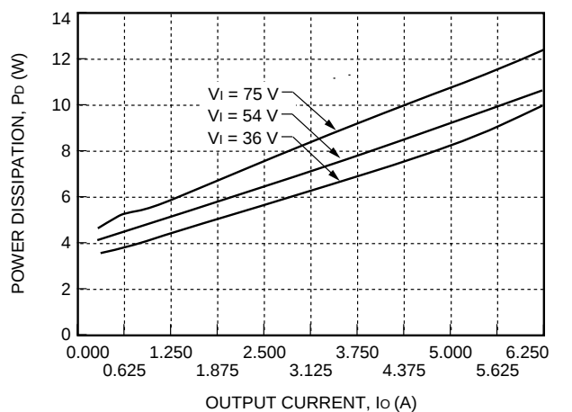
Figure 29. JW075B Power Dissipation vs. Output Current
