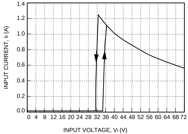
Figure 1. Typical JW050F Input Characteristics at Room Temperature
