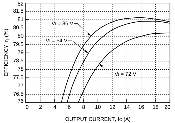
Figure 11. Typical JW100F Converter Efficiency vs. Output Current at Room Temperature
