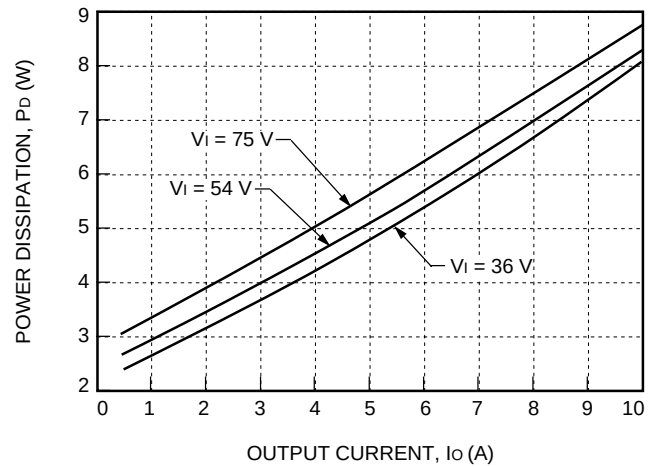
Figure 27. JW050F Power Dissipation vs. Output Current
