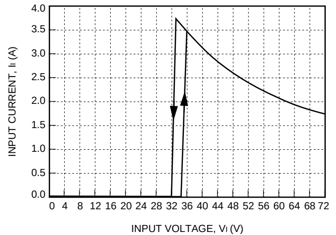
Figure 4. Typical JW150F Input Characteristics at Room Temperature
