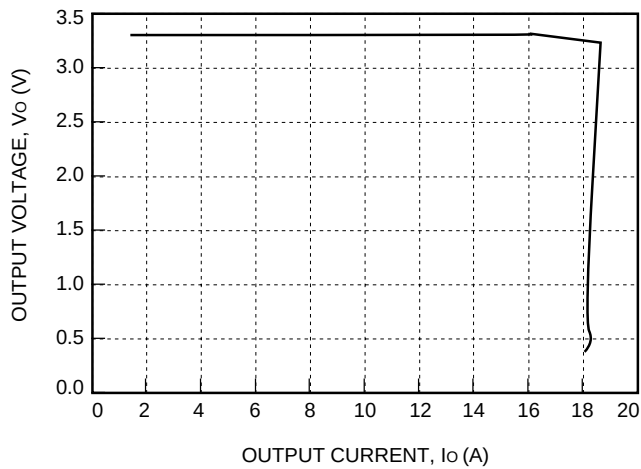
Figure 6. Typical JW075F Output Characteristics at Room Temperature
