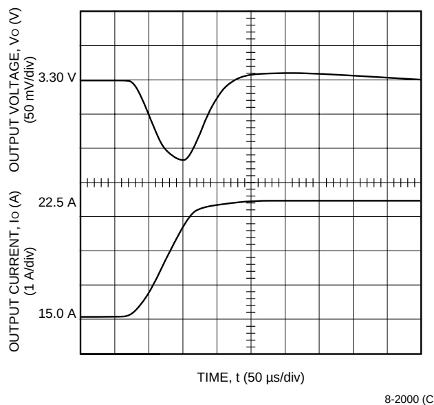
Figure 14. Typical JW150F Transient Response to Step Increase in Load from 50% to 75% of Full Load at Room Temperature and 48 V Input (Waveform Averaged to Eliminate Ripple Component.)
