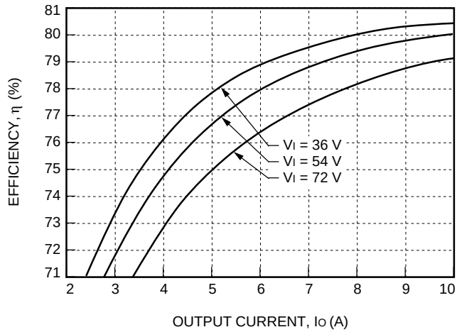
Figure 9. Typical JW050F Converter Efficiency vs. Output Current at Room Temperature
