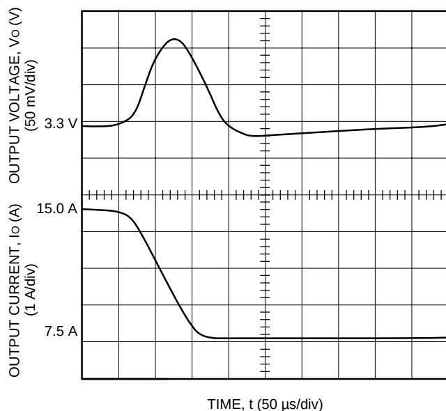
Figure 15. Typical JW150F Transient Response to Step Decrease in Load from 50% to 25% of Full Load at Room Temperature and 48 V Input (Waveform Averaged to Eliminate Ripple Component.)
