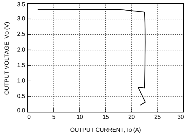
Figure 7. Typical JW100F Output Characteristics at Room Temperature
