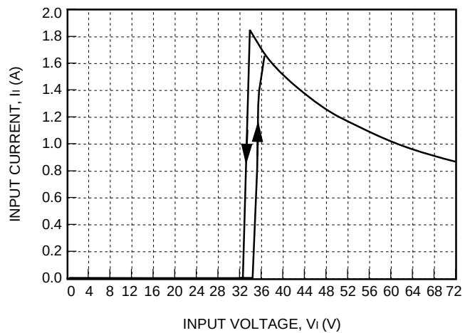
Figure 2. Typical JW075F Input Characteristics at Room Temperature
