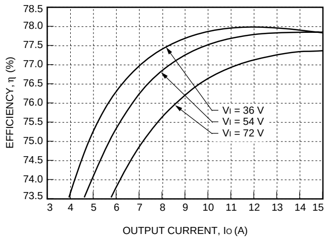
Figure 10. Typical JW075F Converter Efficiency vs. Output Current at Room Temperature
