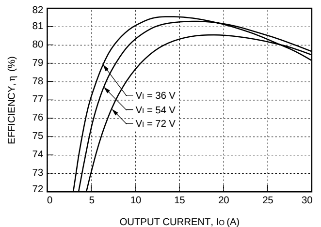
Figure 12. Typical JW150F Converter Efficiency vs. Output Current at Room Temperature
