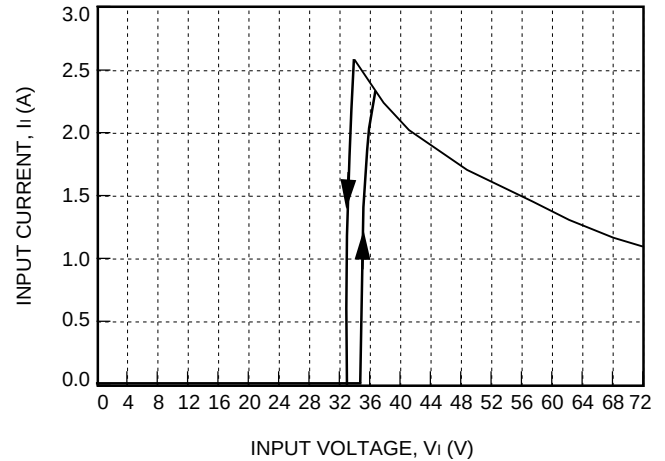
Figure 3. Typical JW100F Input Characteristics at Room Temperature
