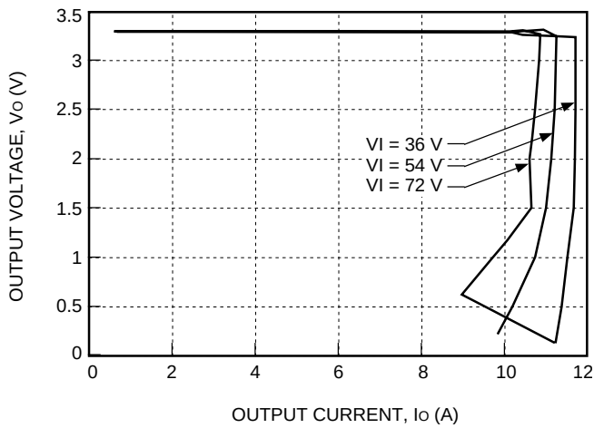
Figure 5. Typical JW050F Output Characteristics at Room Temperature
