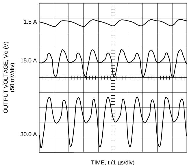
Figure 13. Typical JW150F Output Ripple Voltage at Room Temperature, I_o = Full Load
