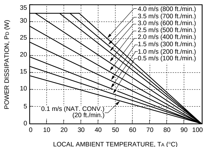
Figure 31. Forced Convection Power Derating with No Heat Sink; Either Orientation
