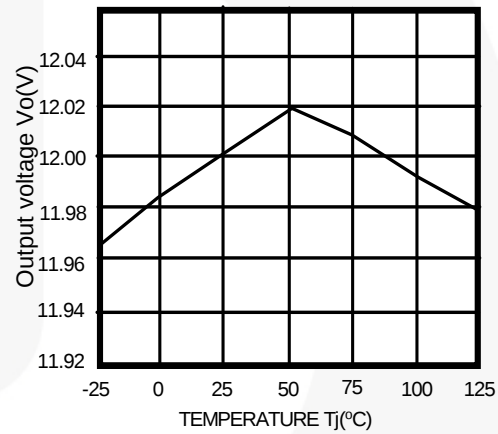
Figure 24. Output Voltage vs. Temperature ( T_j )
