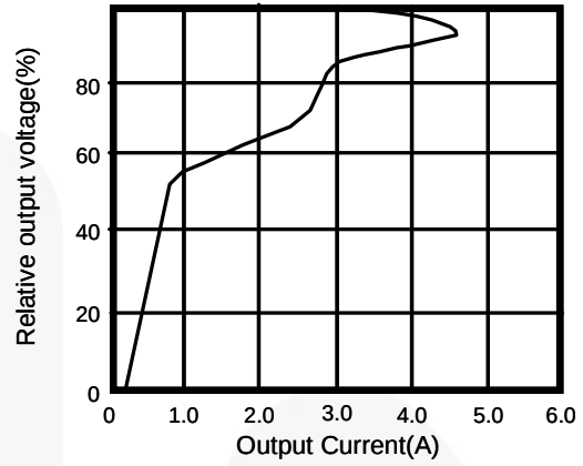
Figure 19. Over-Current Protection Characteristics (Typical Value)
