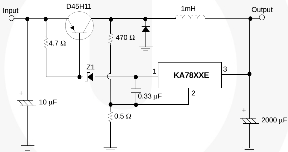
Figure 18. Switching Regulator
