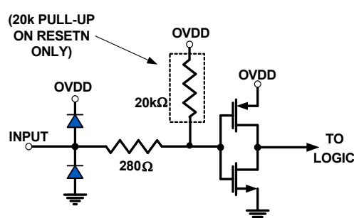
FIGURE 44. DIGITAL INPUTS
