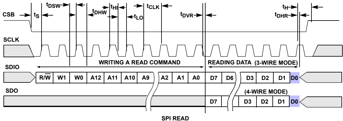
FIGURE 36. SPI READ
