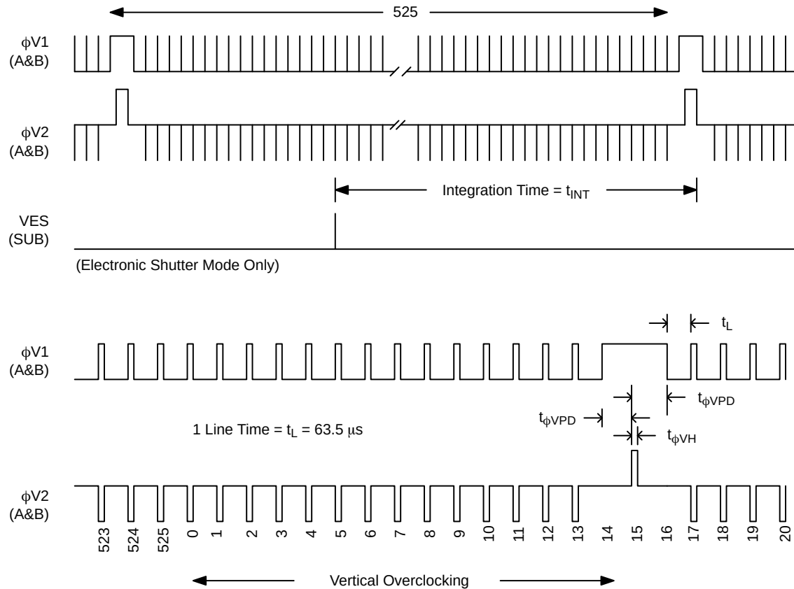
Figure 10. Frame Timing
