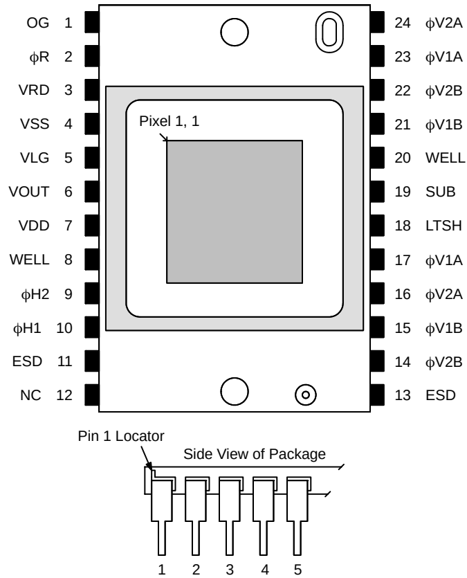
Figure 5. Pin Description
