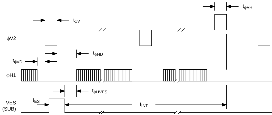
Figure 13. Electronic Shutter Timing
