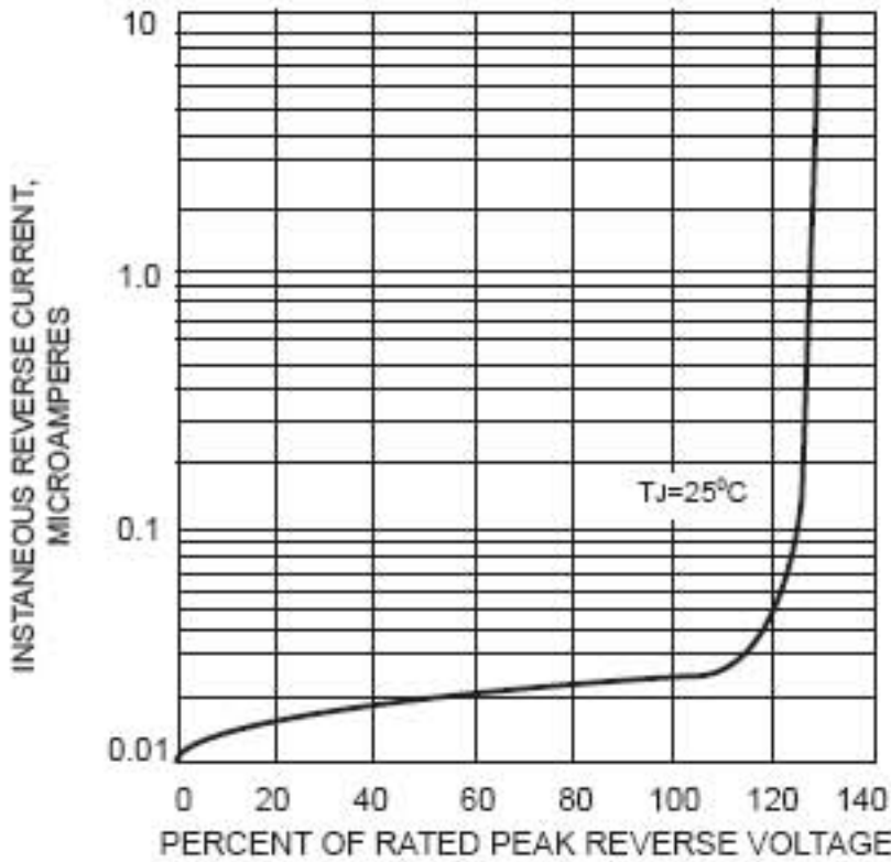
FIG.4 - TYPICAL REVERSE CHARACTERISTICS
