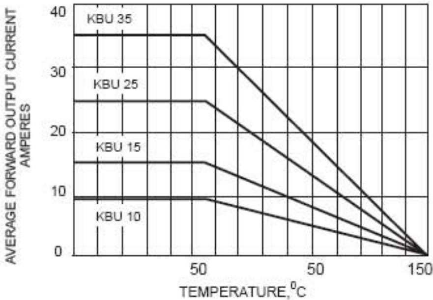
FIG.2 -DERATING CURVE OUTPUT RECTIFIED CURRENT
