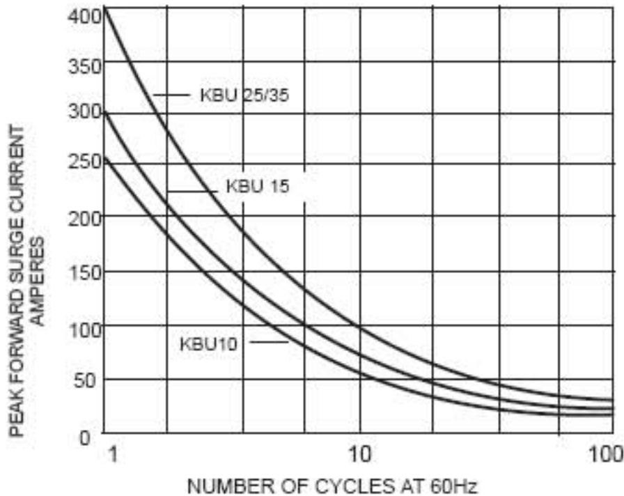
FIG.1 -MAXIMUN FORWARD SURGE CURRENT
