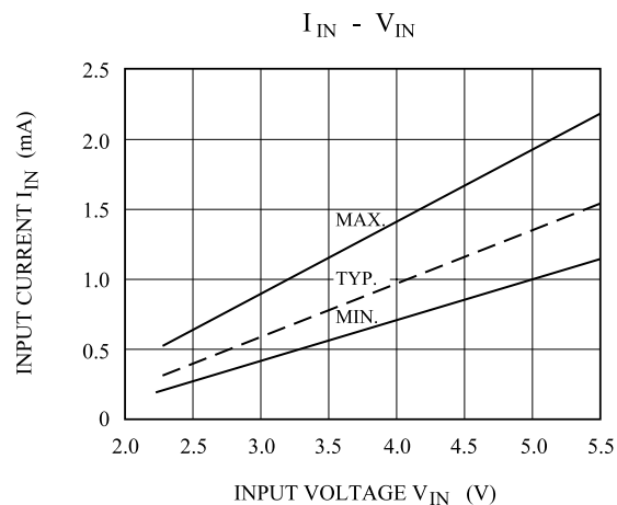
KID65003AP/AF
