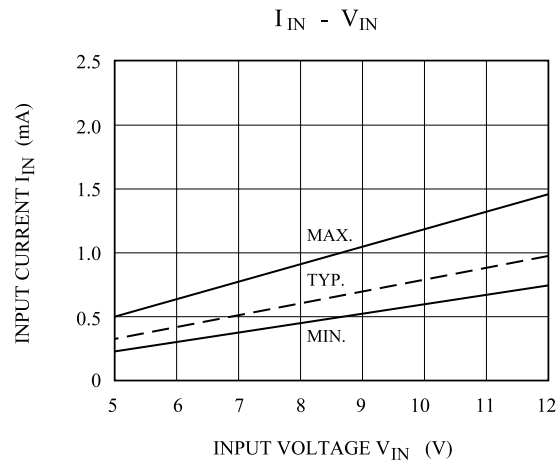
KID65004AP/AF
