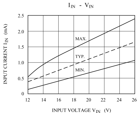
KID65002AP/AF
