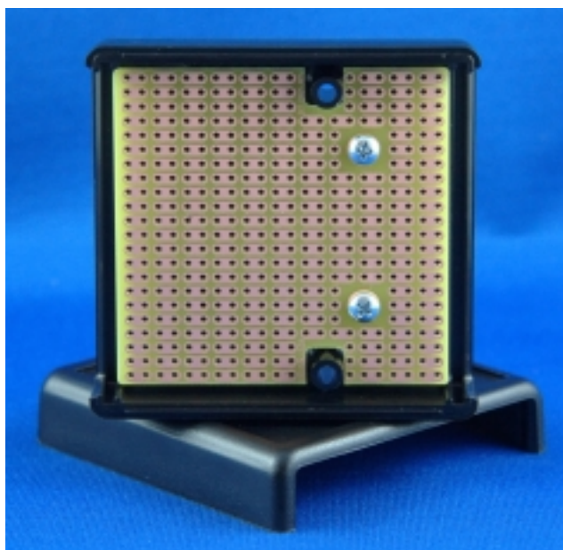
PR1593K Prototyping Board shown with the Hammond 1593KBK box (box not included).
