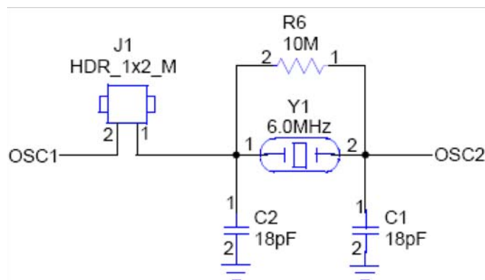
Figure 10. Crystal Circuitry
