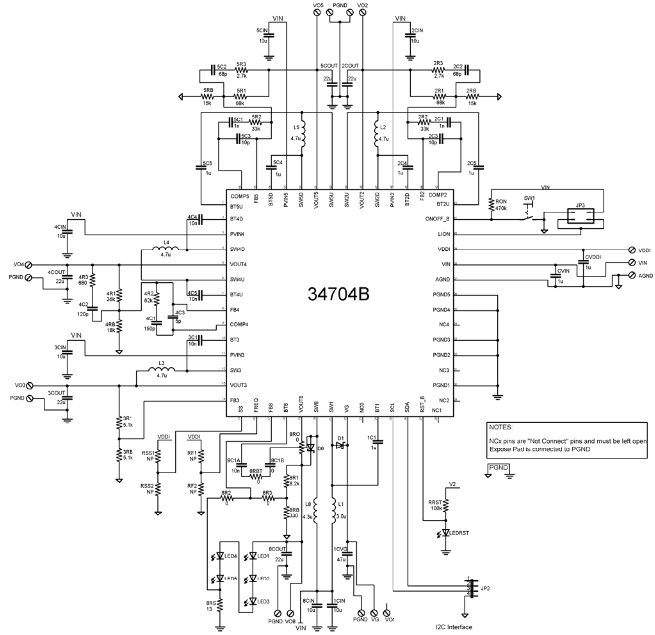
Figure 2. KIT34704BEPEVBE Schematic
