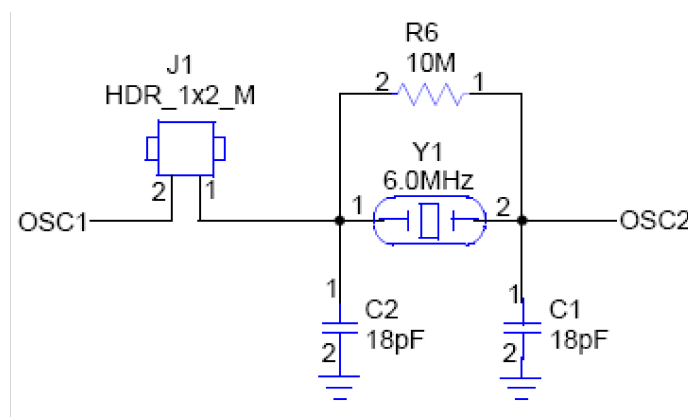
Figure 10. Crystal Circuitry
