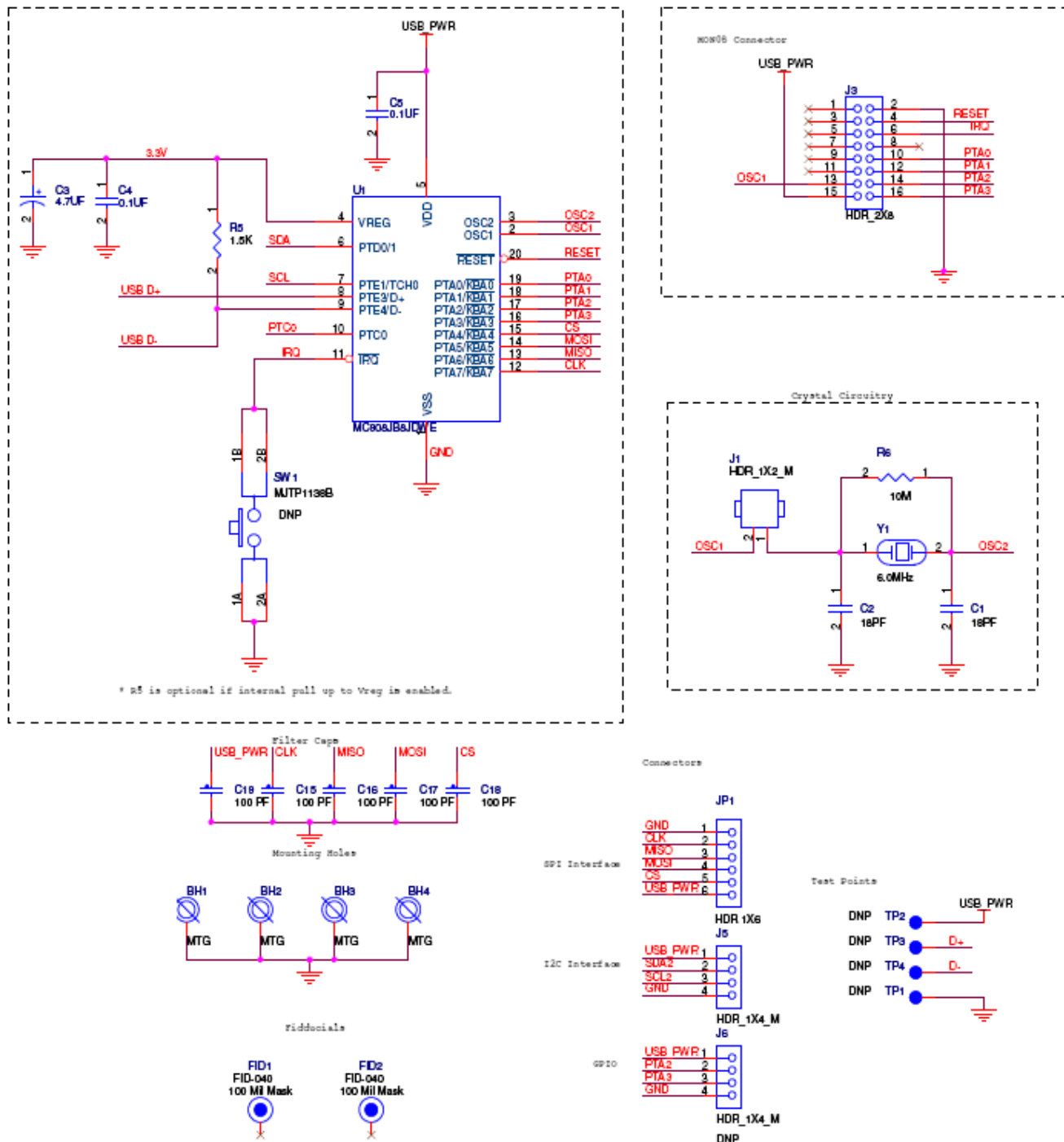
Figure 4. KITUSBI2CEVME Schematic 2
