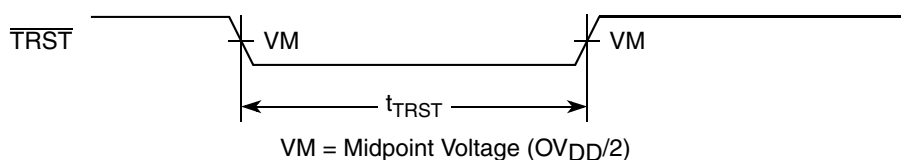
Figure 29. \overline{\text{TRST}} Timing Diagram
