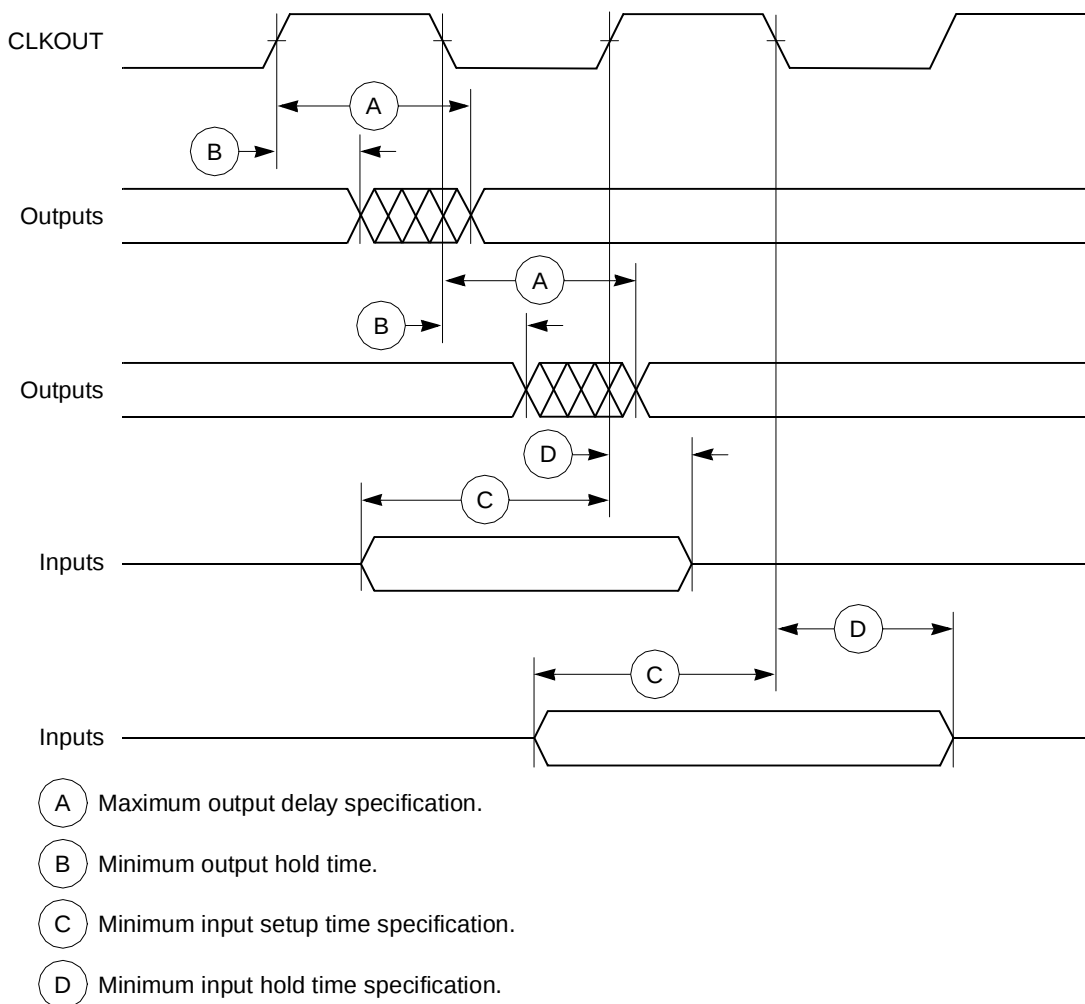
Figure 4. Control Timing
