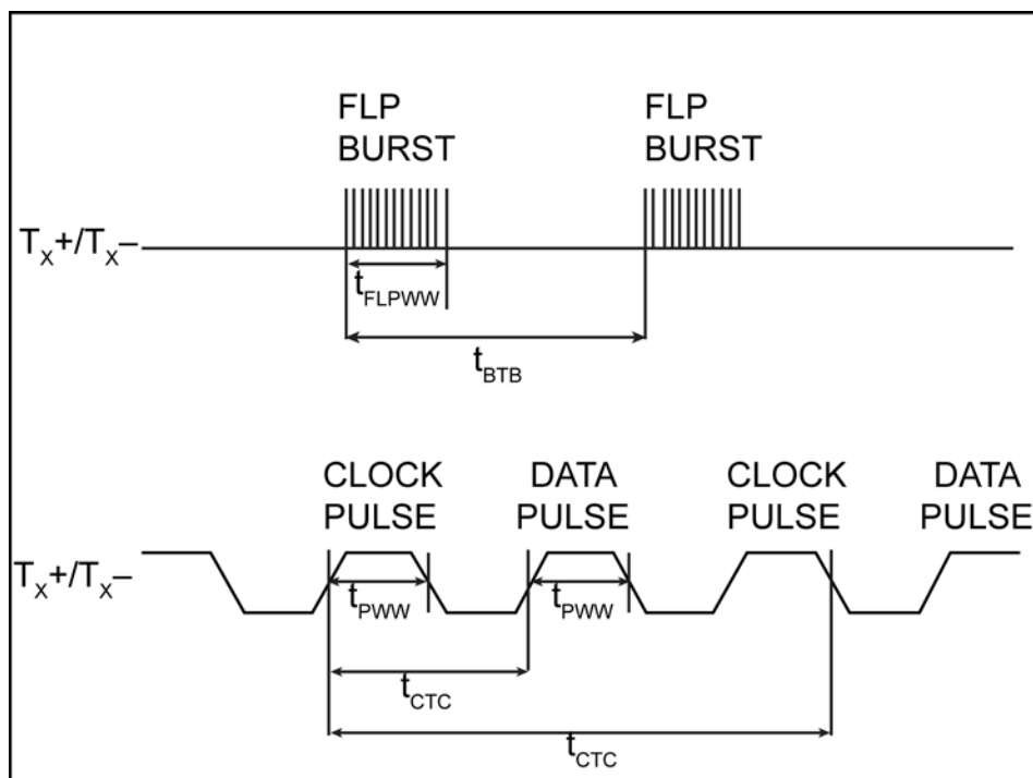
Figure 11. Auto-Negotiation Timing
