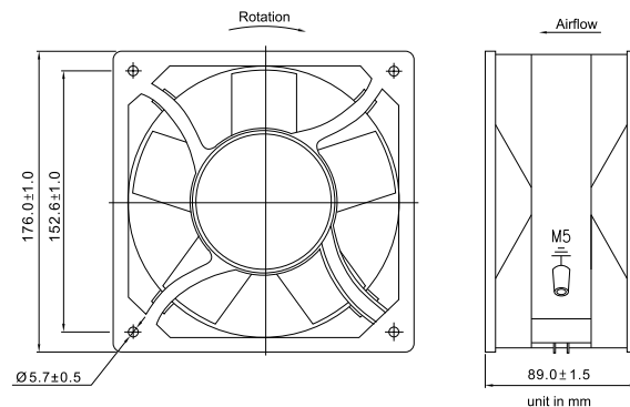
OUTLINE DIMENSIONS
