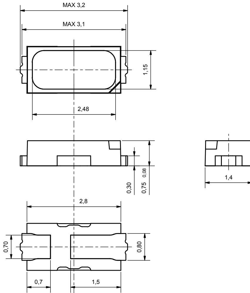
Figure 8: Mechanical dimensions for LUXEON 3014.
