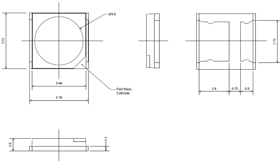
Figure 6b. Mechanical dimensions for L1SP-PRPxx03500000.
