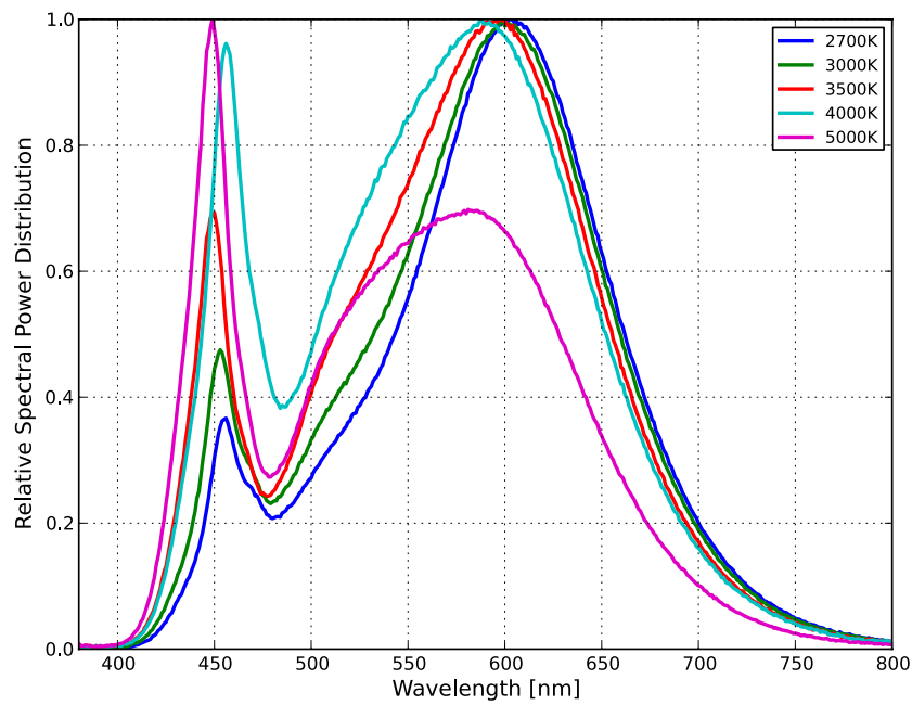
Figure 1b. Typical normalized power vs. wavelength for L1T2-xx800000000000 at 700mA, Tj=85°C.
