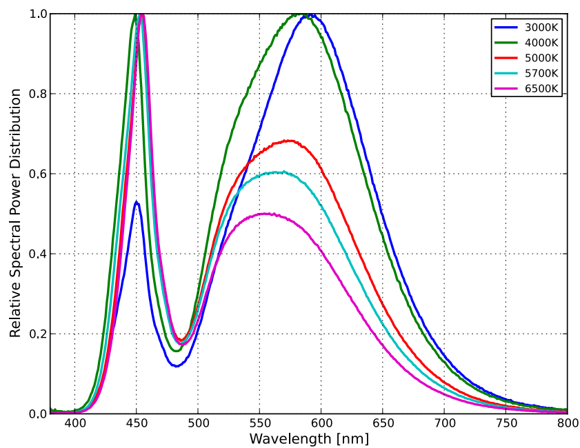
Figure 1a. Typical normalized power vs. wavelength for L1T2-xx700000000000 at 700mA, Tj=85°C.
