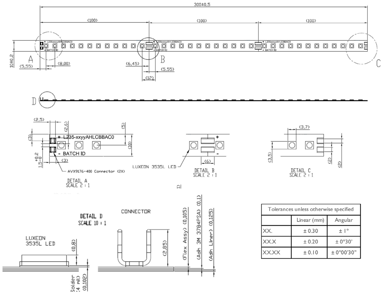
Figure 10: Mechanical dimensions for L235-xyyAHLCCBBAC0.
