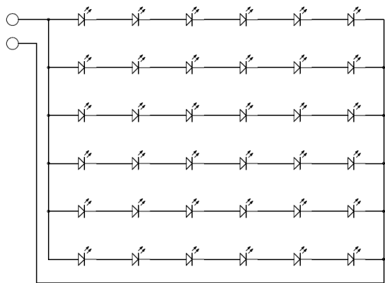
Figure 9: Electrical circuit diagram for L235-xyyAHLCBAA0..
