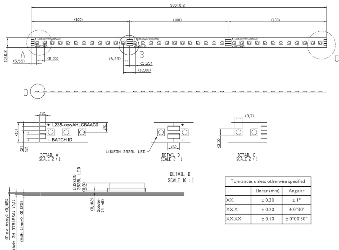
Figure 8: Mechanical dimensions for L235-xyyAHLCBAA0.
