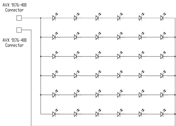
Figure 11. Electrical circuit diagram for L235-xyyAHLCCBBAC0.
