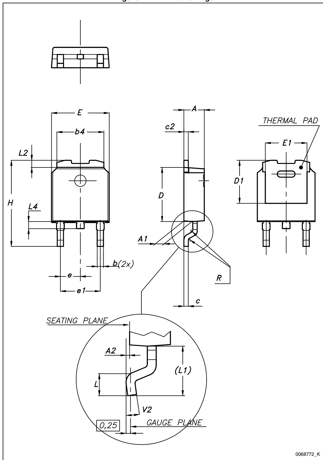
Figure 12. DPAK drawings
