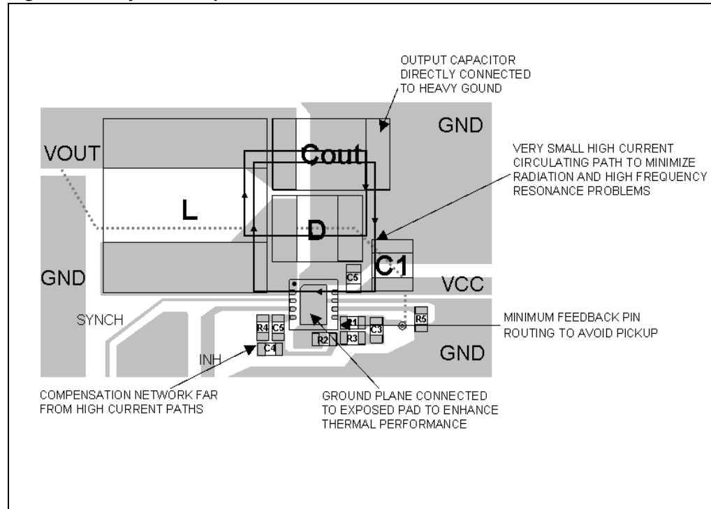
Figure 18. Layout example
