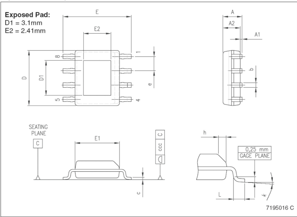
Figure 35. Package dimensions
