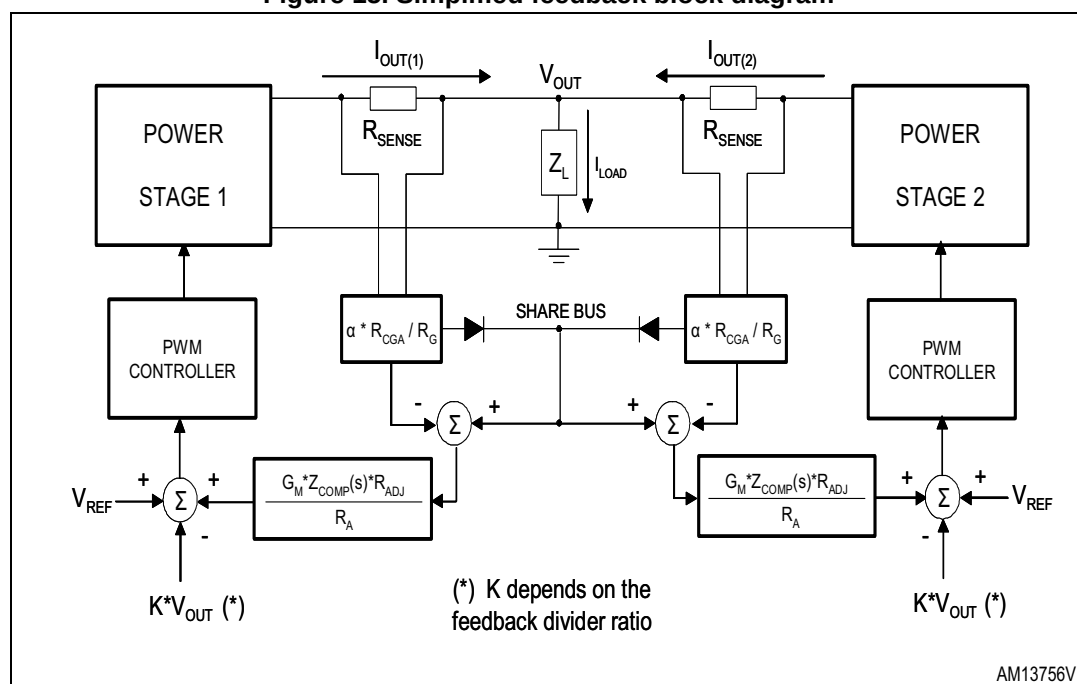
Figure 15. Simplified feedback block diagram
