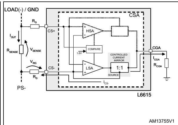
Figure 14. Current sense (low-side)
