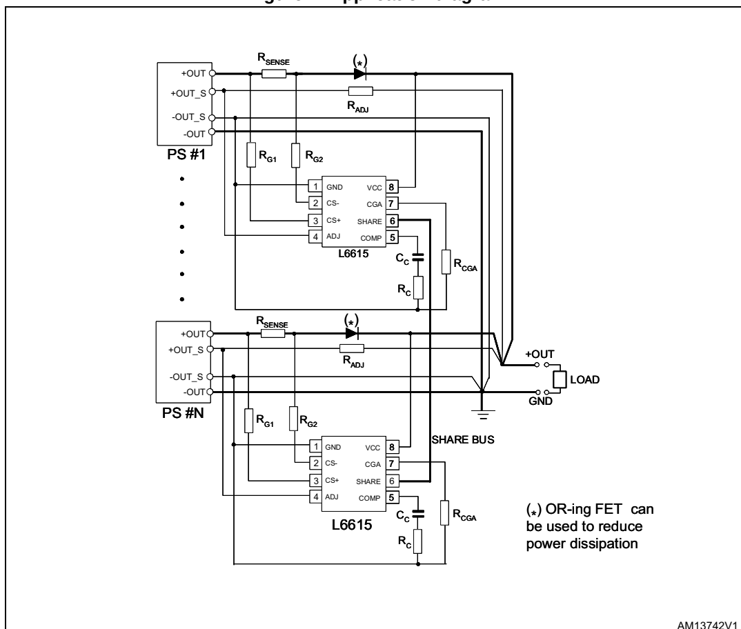
Figure 1. Application diagram
