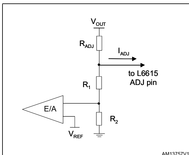
Figure 16. ADJ network
