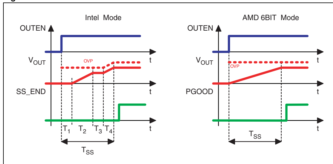
Figure 15. Soft-start
