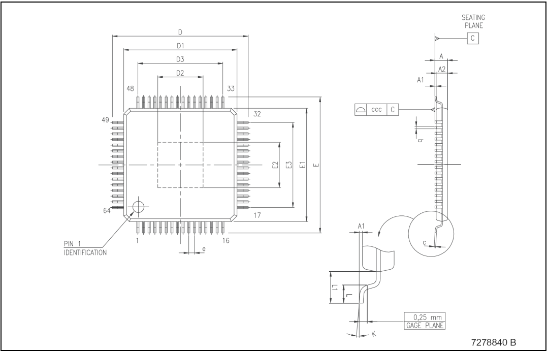
Figure 29. Package dimensions
