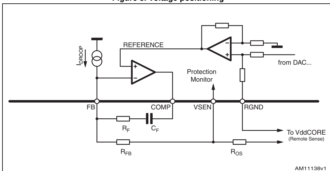
Figure 5. Voltage positioning
