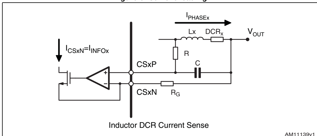
Figure 6. Current reading
