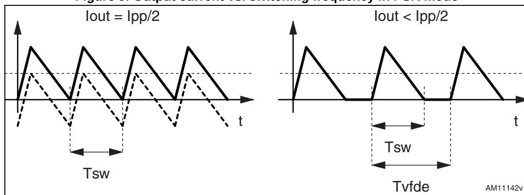
Figure 9. Output current vs. switching frequency in PSK mode
