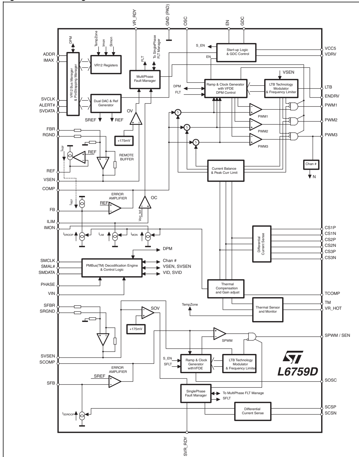
Figure 3. Block diagram
