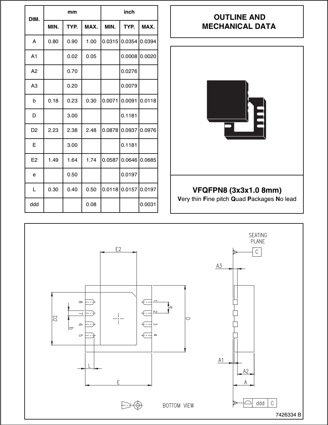
Figure 5. VFQFPN8 mechanical data & package dimensions
