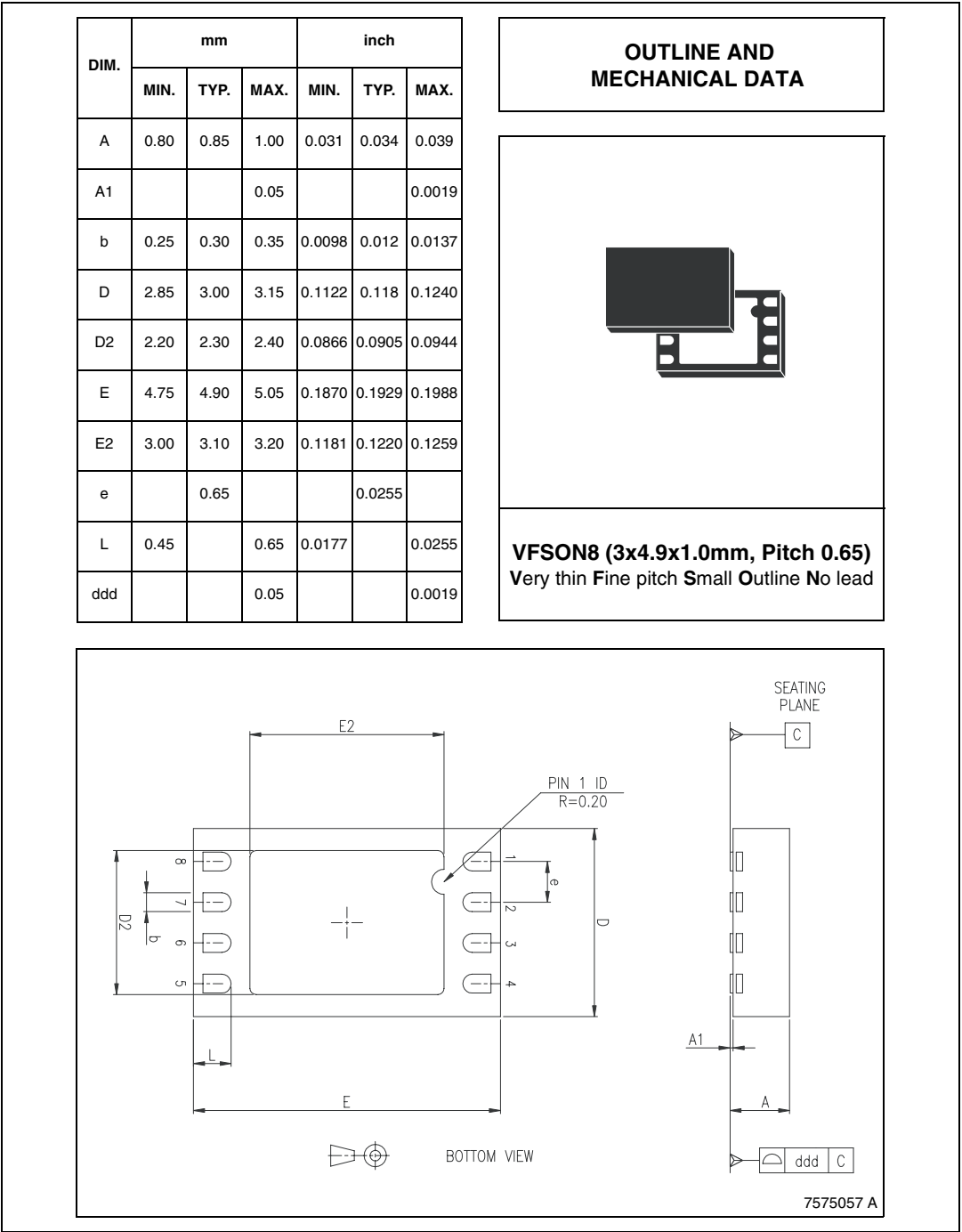
Figure 4. VFSON8 mechanical data & package dimensions
