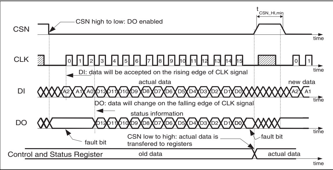
Figure 10. Transfer timing diagram
