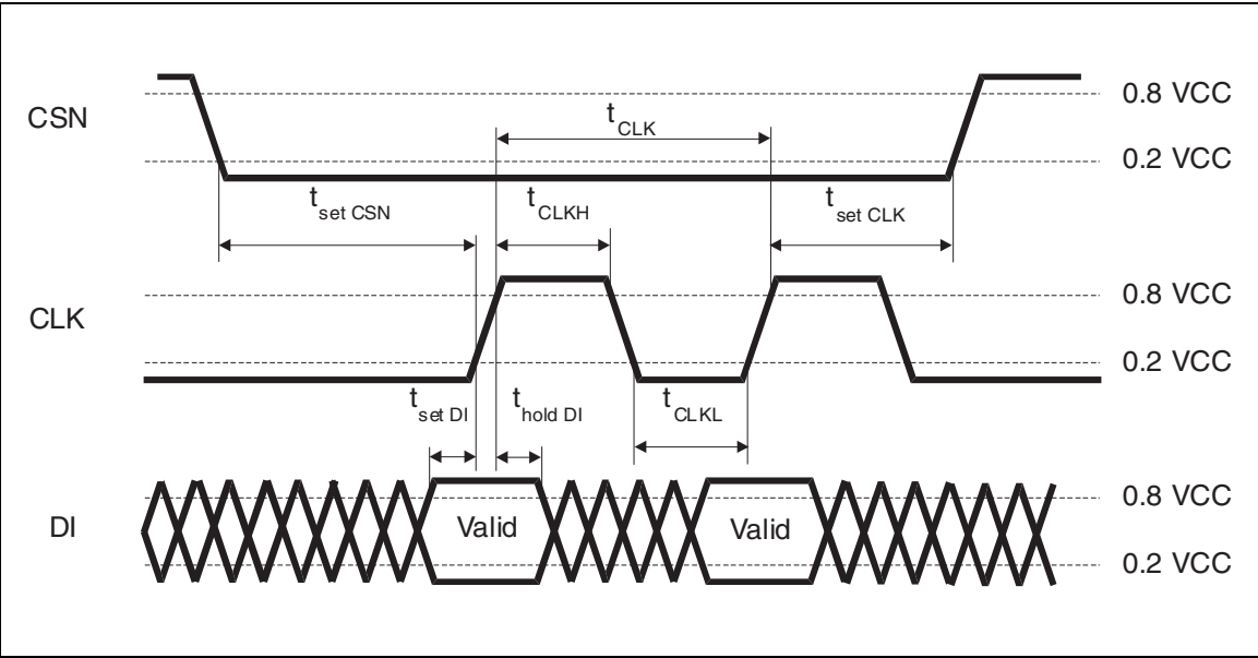
Figure 11. Input timing
