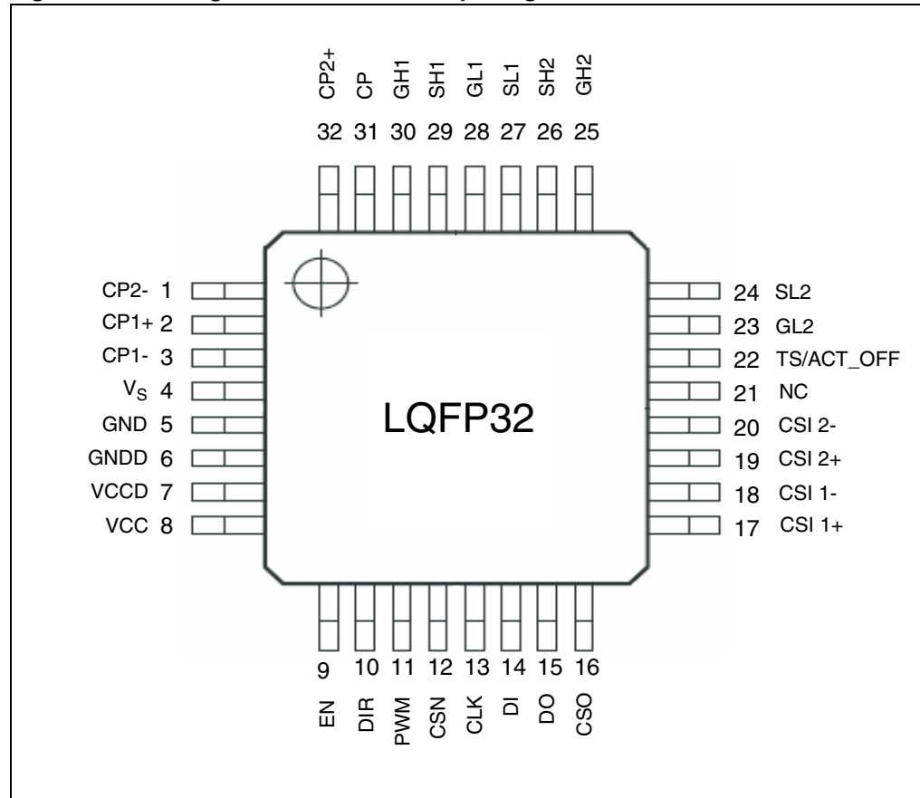
Figure 3. Pinning of device in LQFP-32 package
