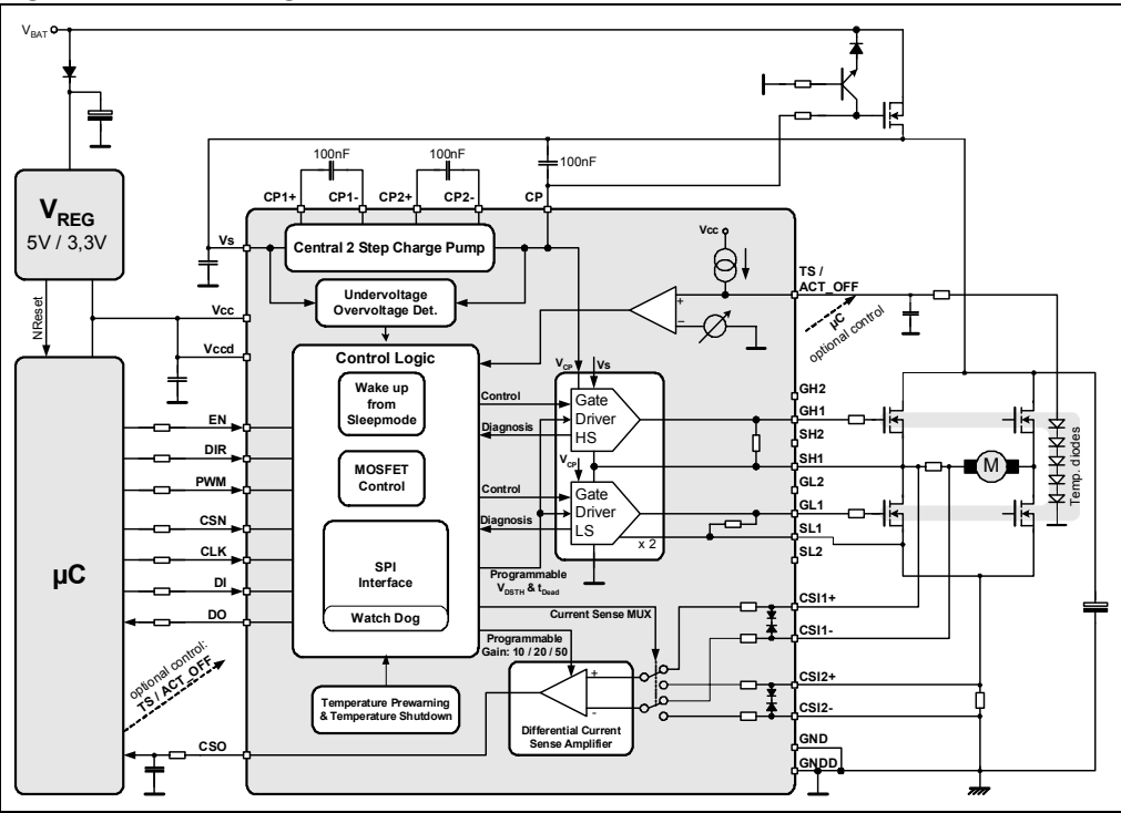
Figure 1. Block diagram
