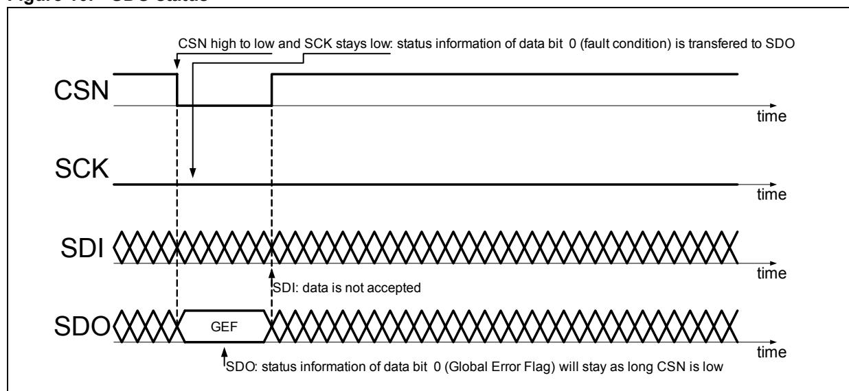
Figure 10. SDO status
