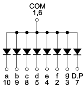
Anode Common
