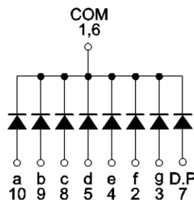
Cathode Common
