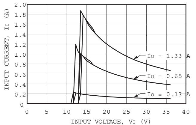
Figure 4. LC020C Typical Input Characteristics, T_A = 25^\circ\text{C}
