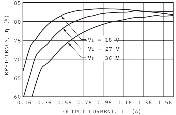
Figure 11. LC020B Typical Converter Efficiency vs. Output Current, TA = 25 °C
