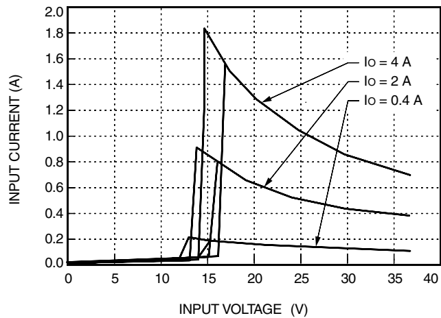
Figure 2. LC020A Typical Input Characteristics, T_A = 25^\circ\text{C}
