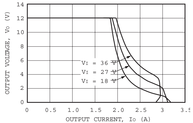
Figure 7. LC020B Typical Output Characteristics, T_A = 25^\circ\text{C}
