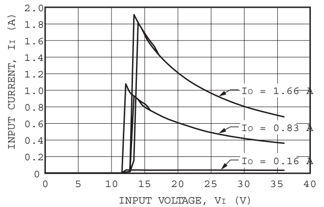
Figure 3. LC020B Typical Input Characteristics, T_A = 25^\circ\text{C}
