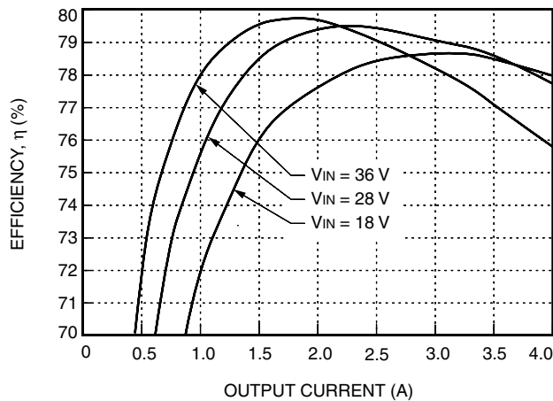
Figure 10. LC020A Typical Converter Efficiency vs. Output Current, TA = 25 °C
