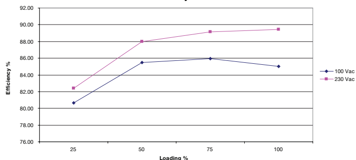
LCM1500Q Efficiency Without the 5 Vsb
