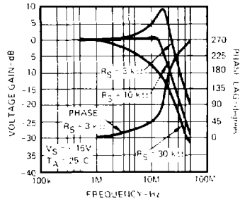
Voltage Gain
