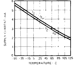
Supply Current
