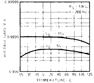
Voltage Gain
