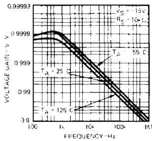
Voltage Gain
