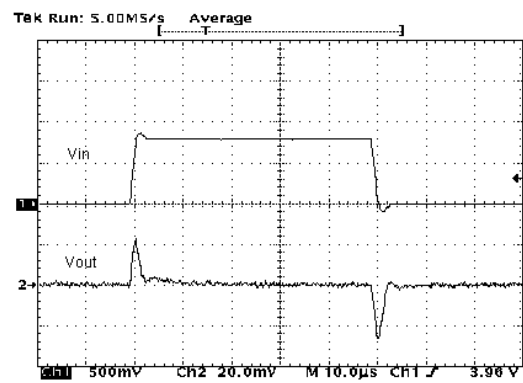
Figure 13. Line transient
