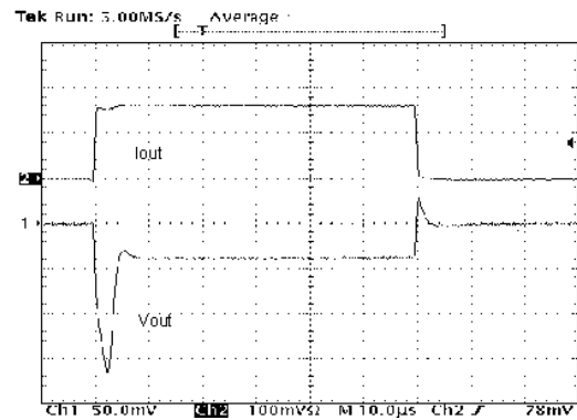
Figure 15. Load transient
