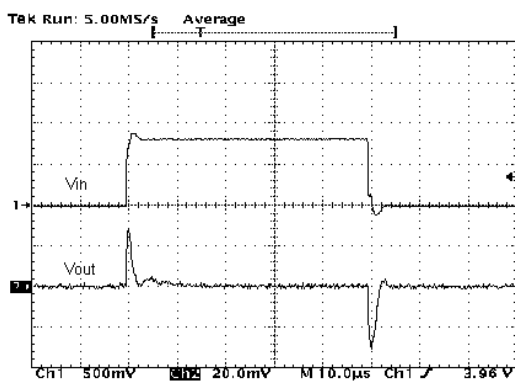
Figure 12. Line transient
