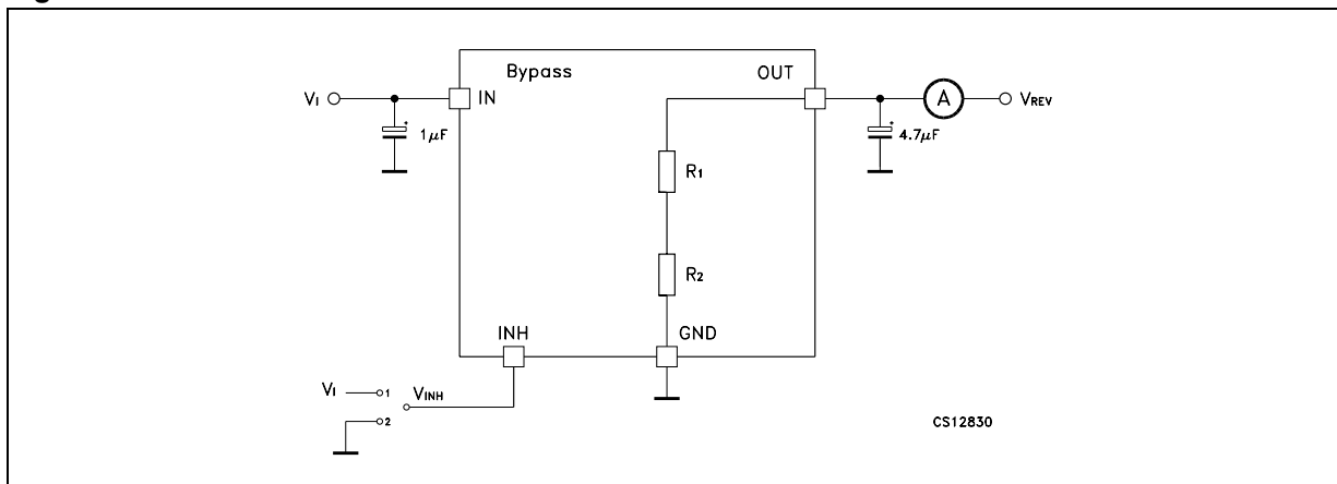
Figure 16. Reverse current test circuit
