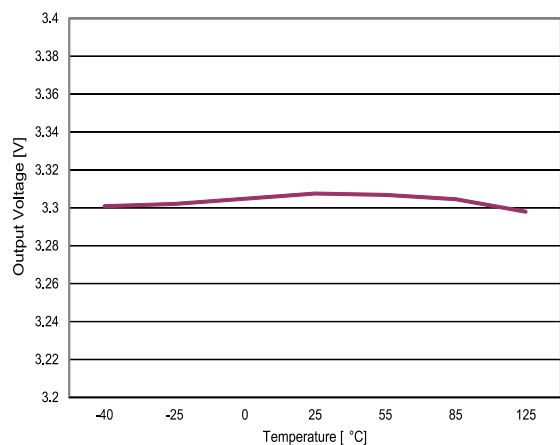
Figure 4: Output voltage vs. temperature ( I_{OUT} = 1 \text{ mA} )
