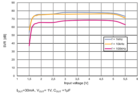
Figure 15: Supply voltage rejection vs. input voltage
